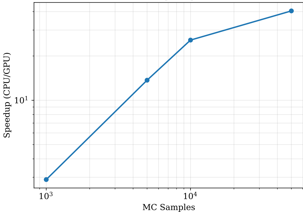
MC Speedup
