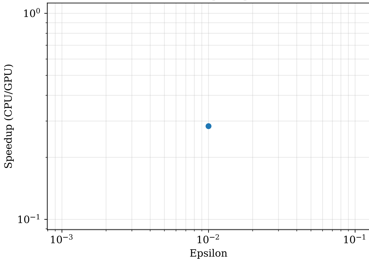
MLMC Speedup
