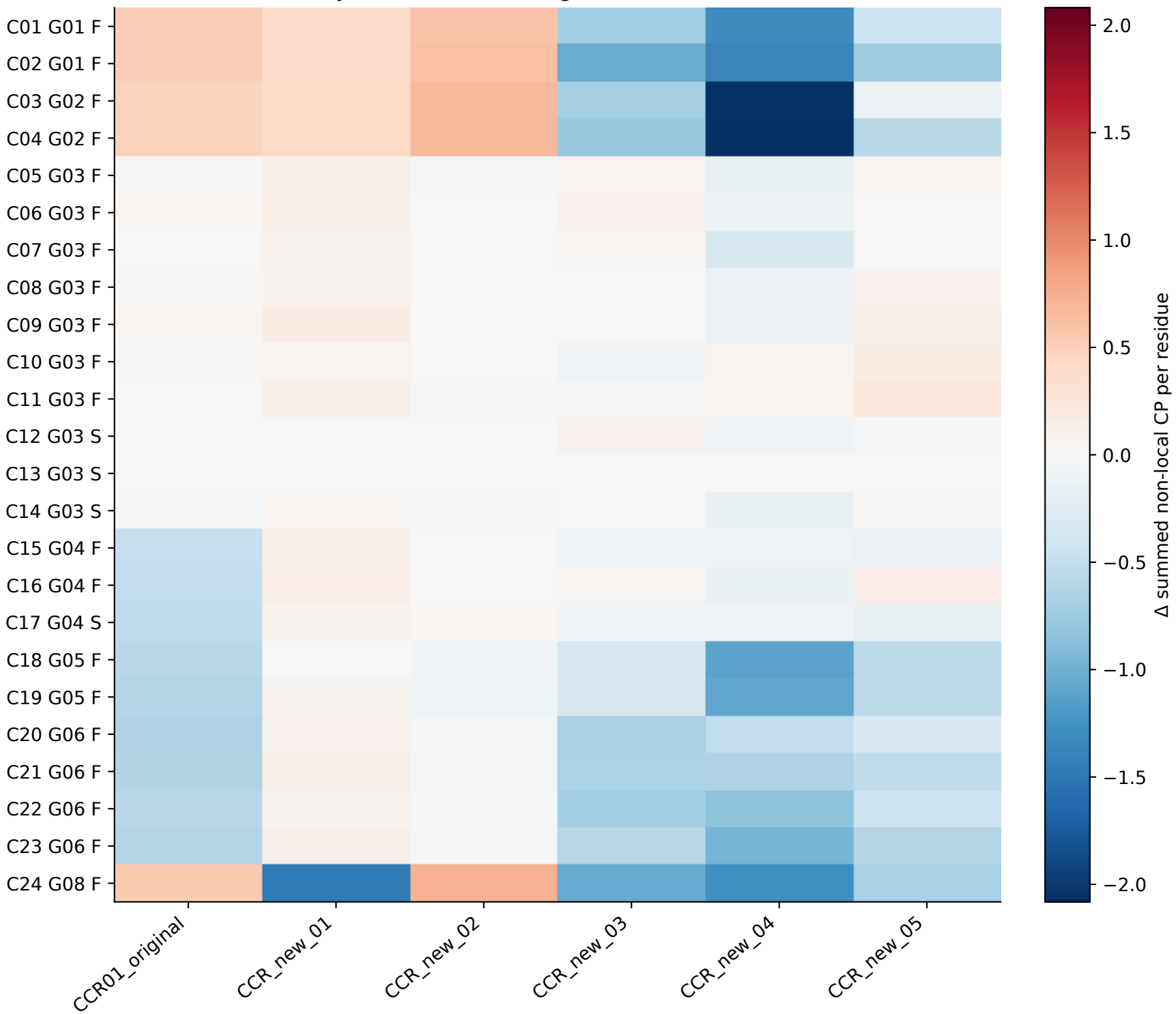
CCR density difference from original 512-aa success reference
