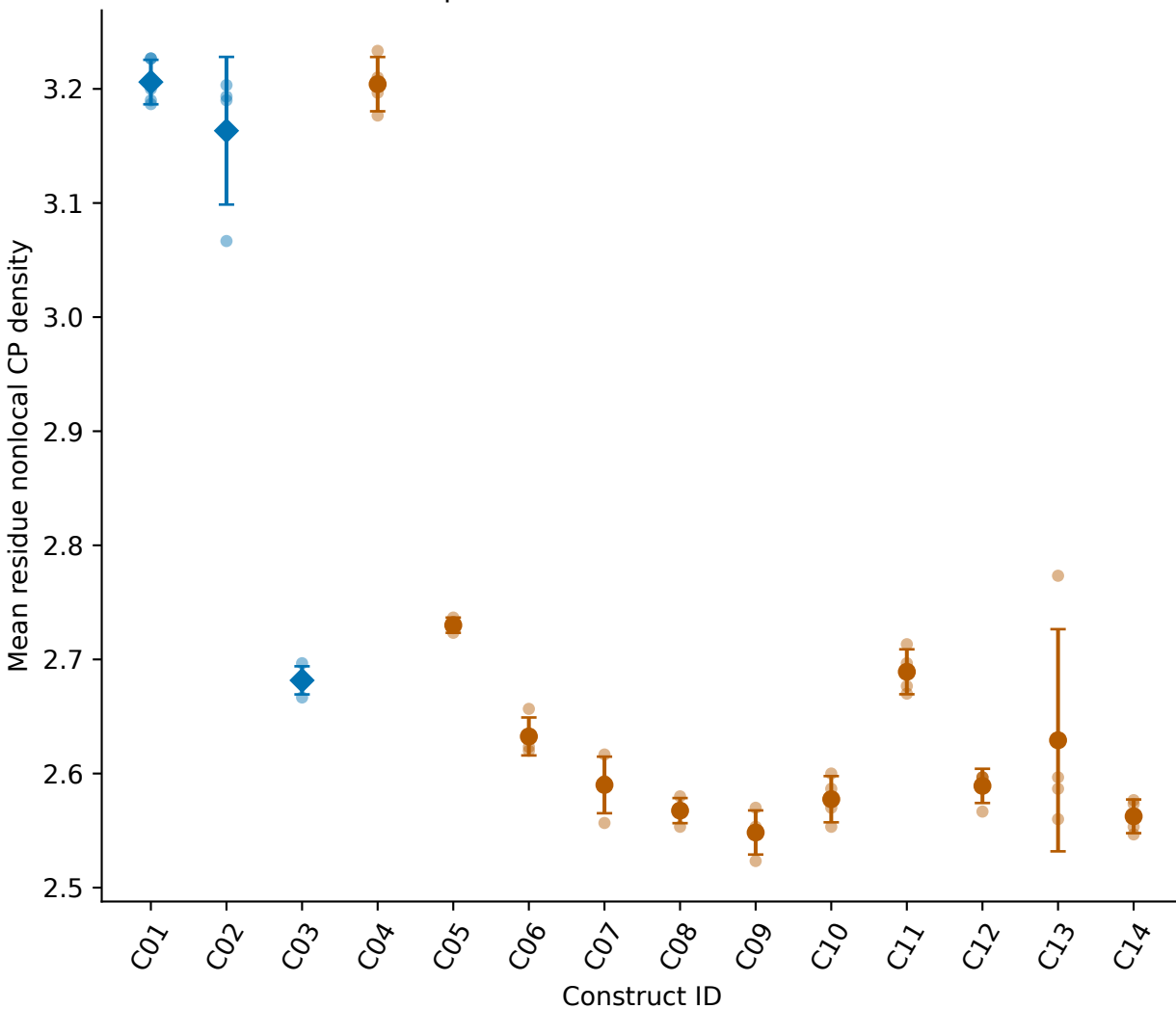
CCR01 | reference residues 178,179,180
