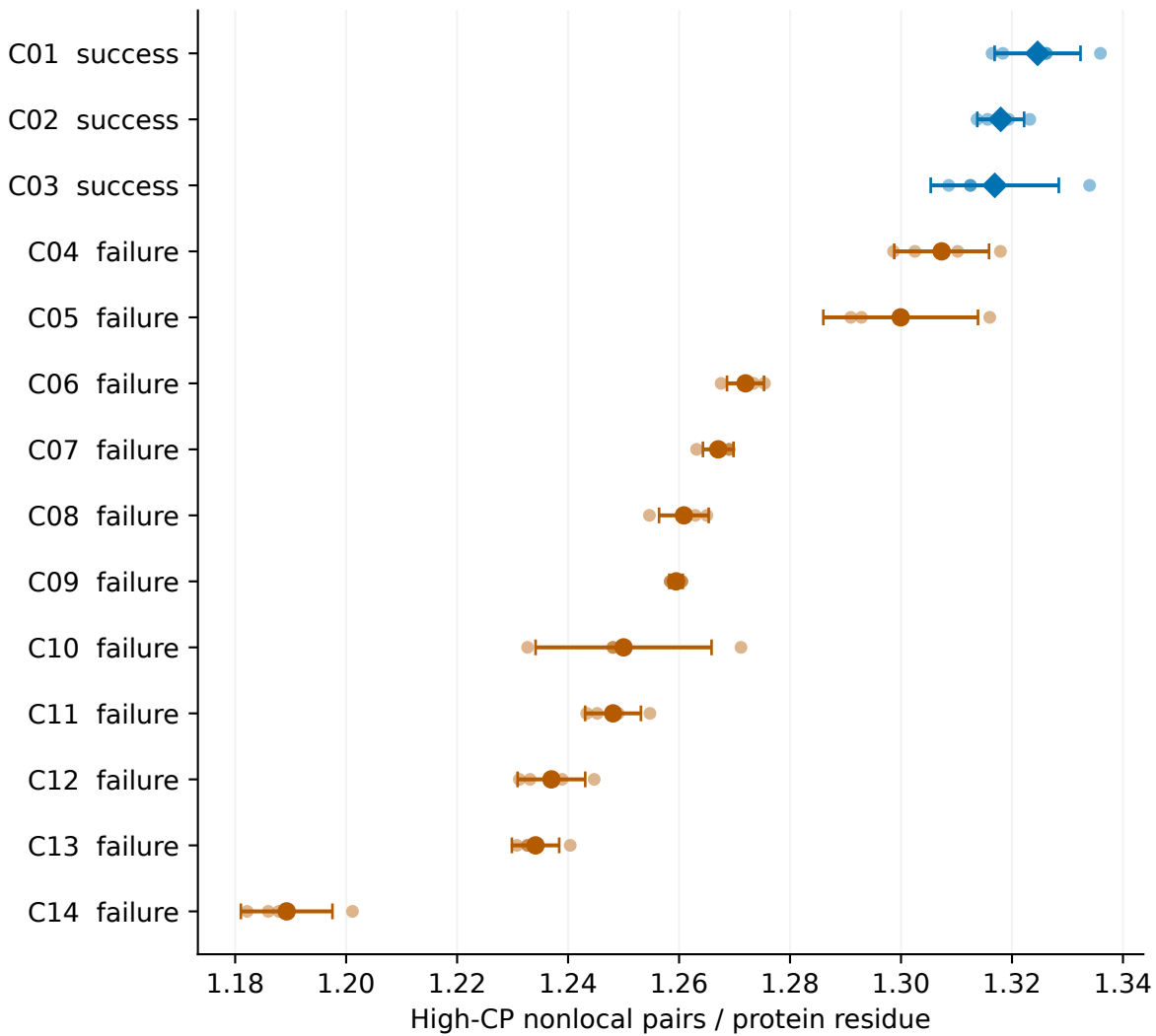
A Protein internal contacts
