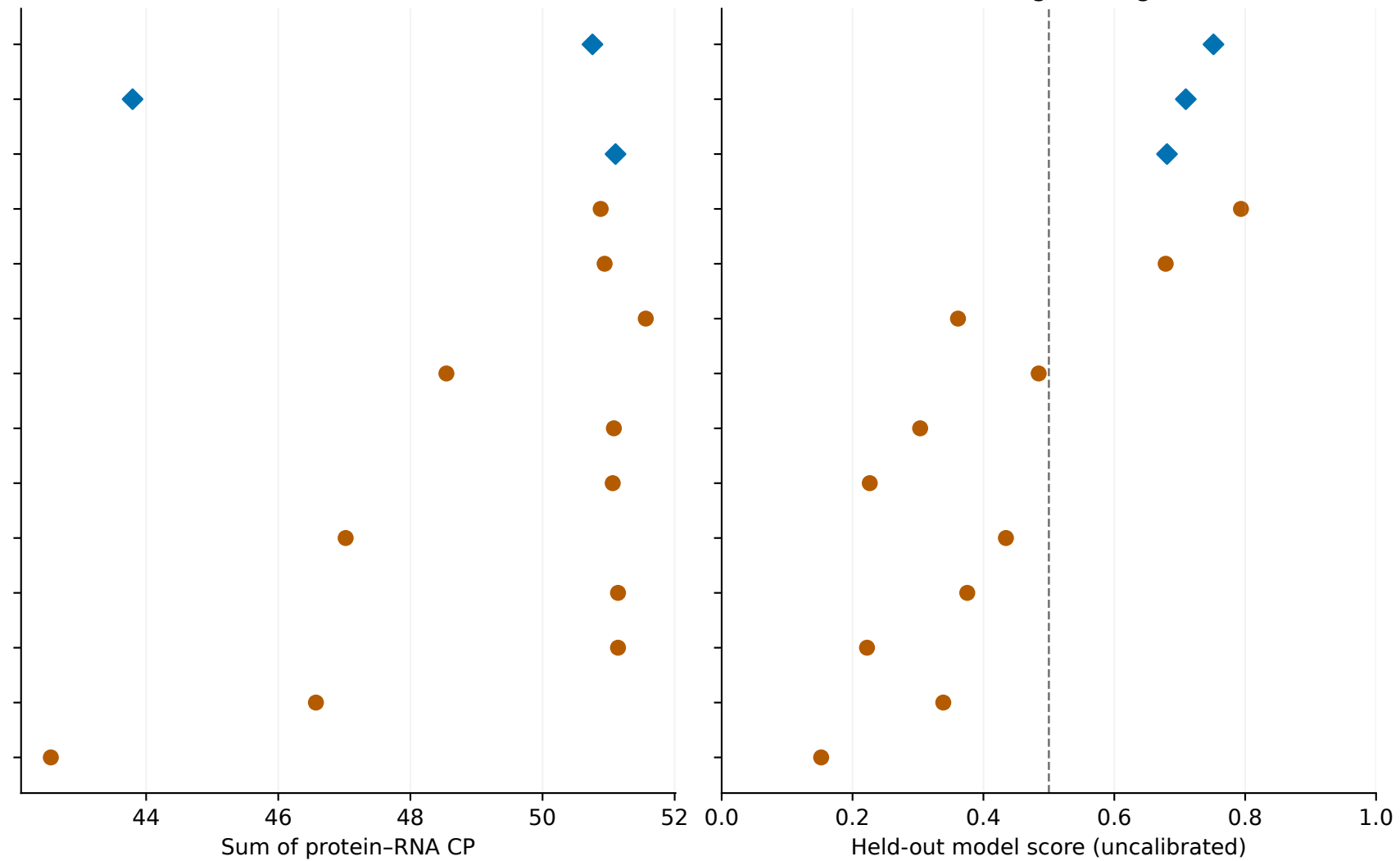
B Protein-RNA contacts
