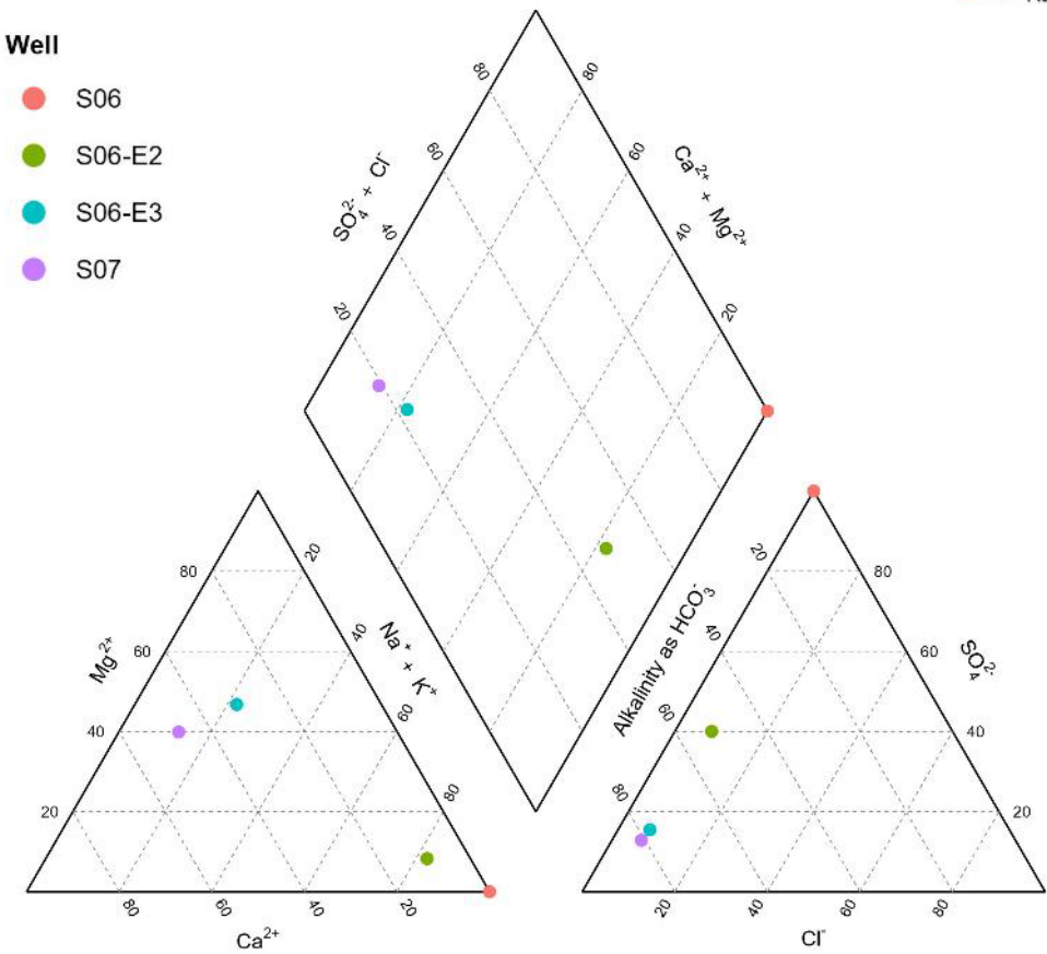
Piper Plot - mean concentration
