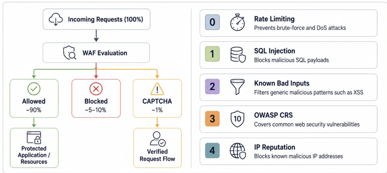
Figure 5.14: AWS Web Application Firewall (WAF) deployment architecture protecting the BK-MInD ALB.
