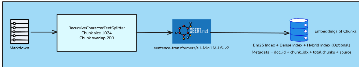
Figure 5.9: Textual Chunking and Embedding.
