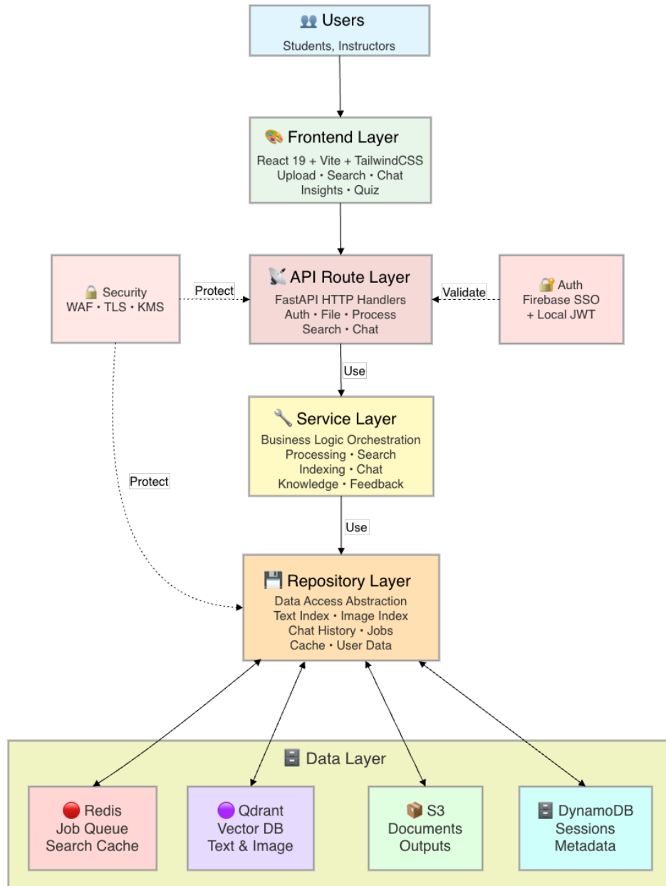
Figure 4.1: High-Level Architecture.
