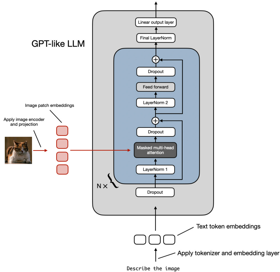
Figure 2.4: Cross-attention.
