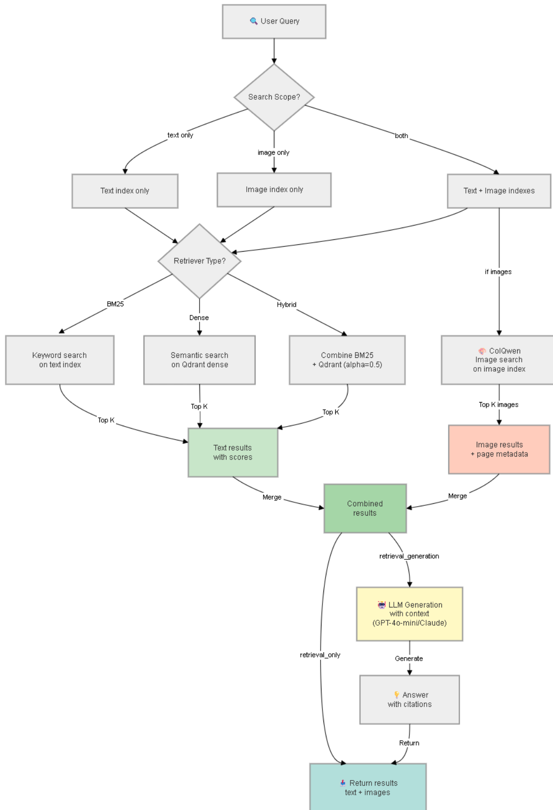
Figure 5.11: Search and Retrieval Pipeline Flow.
