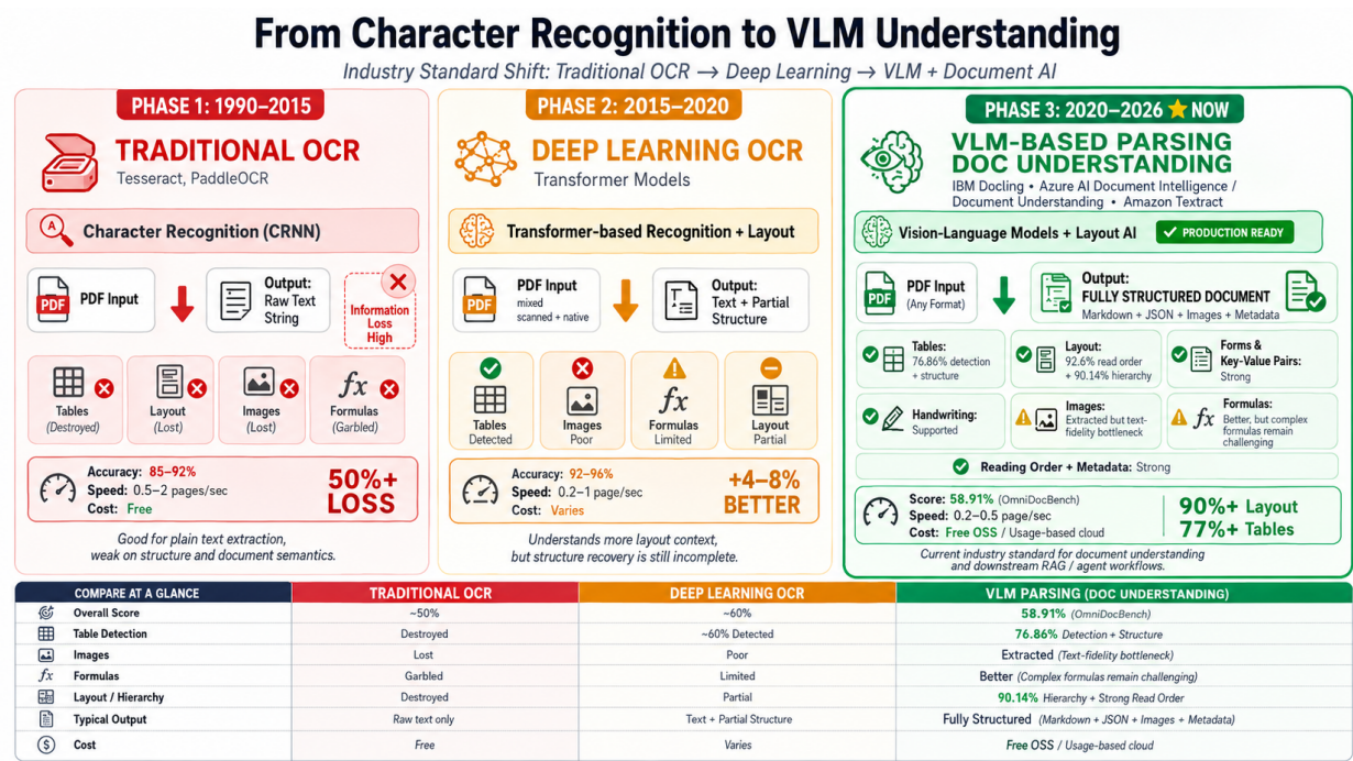
Figure C.3: Three generations of document parsing: OCR evolution.
