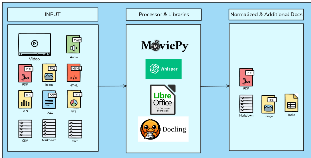
Figure 4.2: Data Processing Pipeline Normalization Stage.
