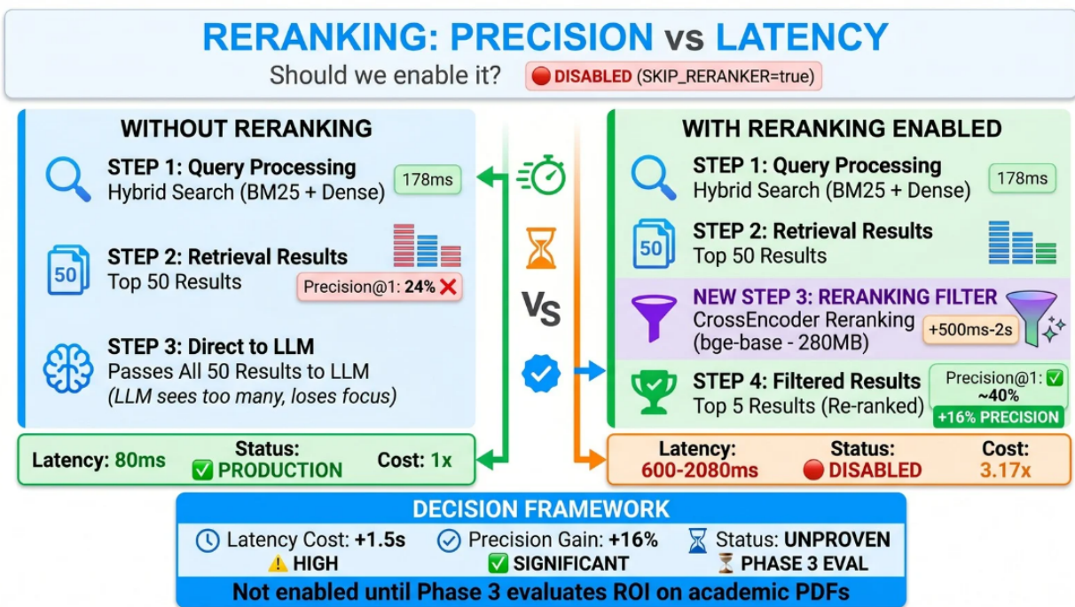
Figure C.1: Reranking trade-off: precision vs. latency comparison.
