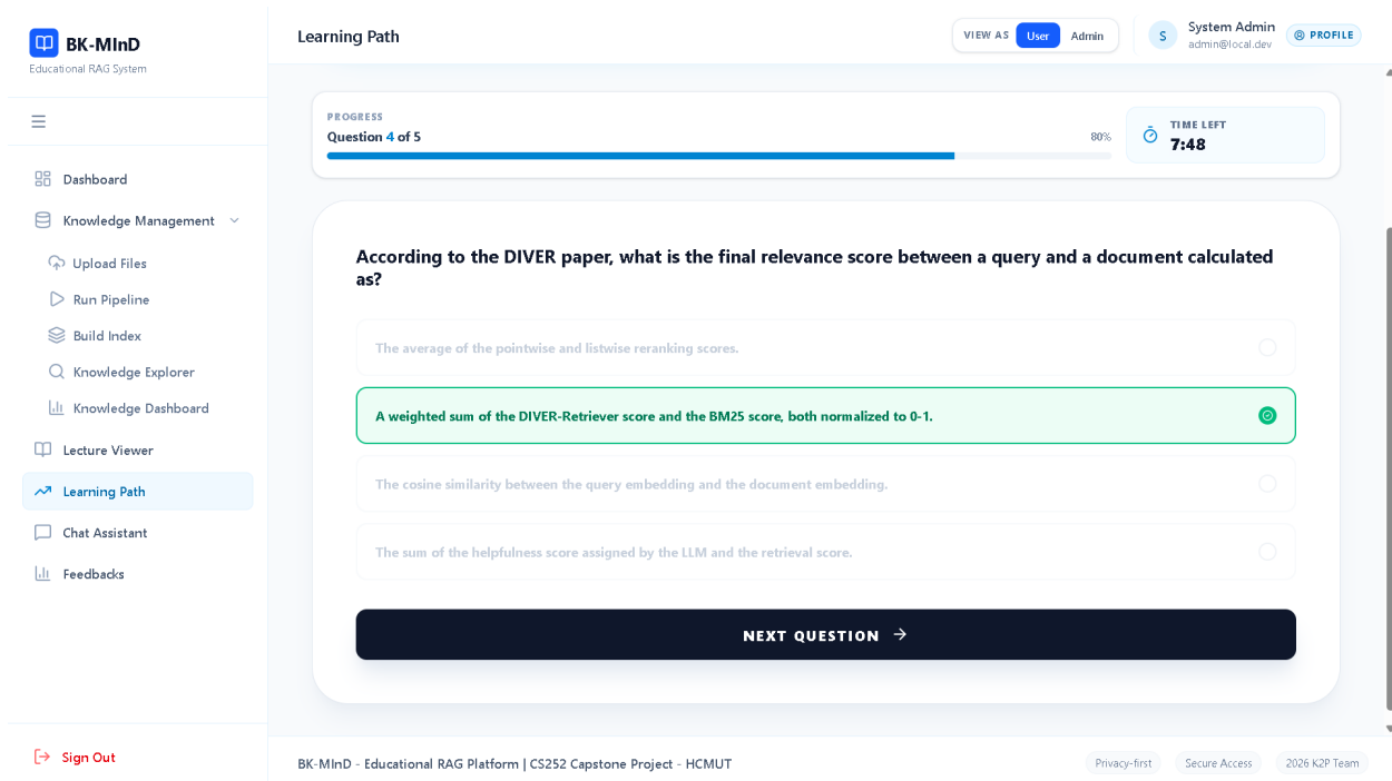
Figure B.9: Multiple Choice Questions: AI generates quiz questions from any lecture. Adjust difficulty, number of questions, and include explanations.
