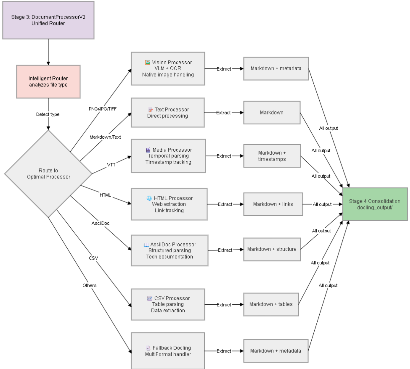
Figure 5.5: DocumentProcessorV2 Unified Router.
