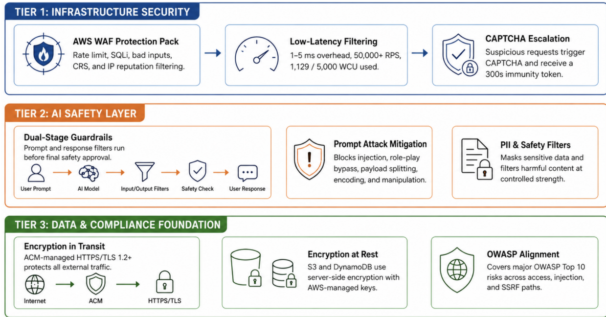
Figure 4.5: BK-MInD Three-Tier Security Architecture.
