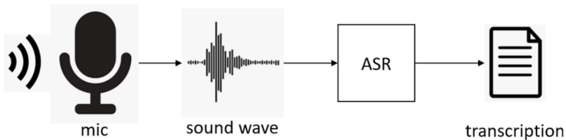
Figure 2.1: ASR pipeline.
