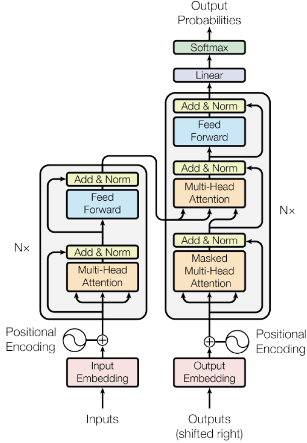
Figure 2.3: Transformer Architecture.
