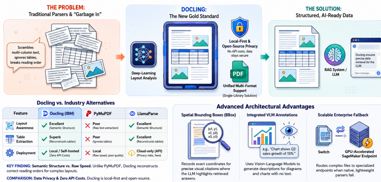
Figure C.4: Docling parser selection criteria and comparison framework.
