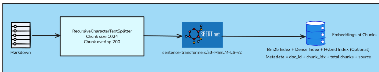
Figure 5.5: Textual Chunking and Embedding.
