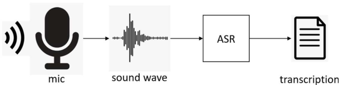
Figure 2.1: ASR pipeline [9]
