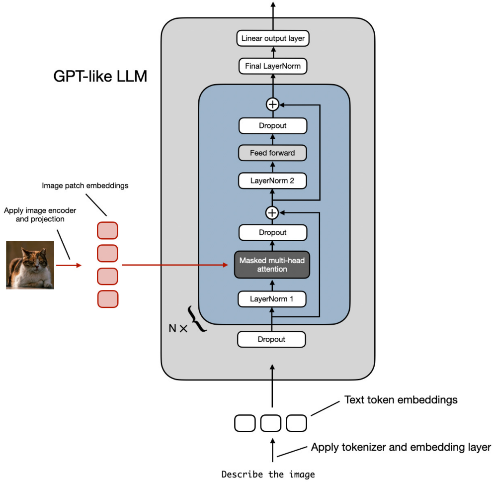
Figure 2.4: Cross-attention [45].
