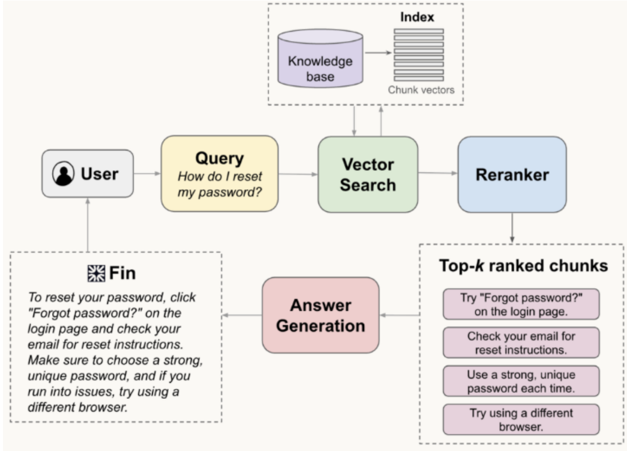
Figure 2.8: Reranker [138].
