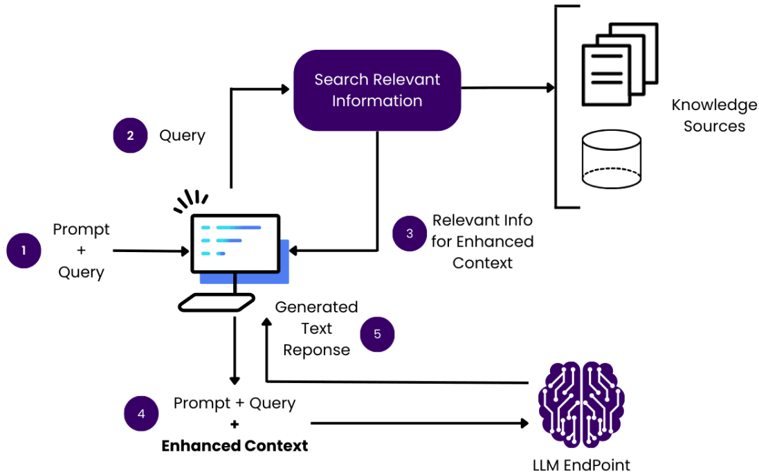
Figure 2.9: Augmentation [143]
