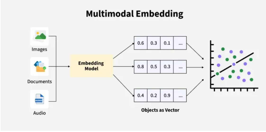
Figure 2.5: Multimodal embedding [47].
