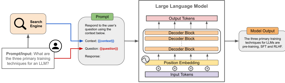
Figure 2.10: Generation [147]
