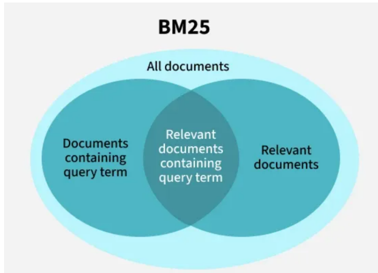
Figure 2.7: BM25 [132].
