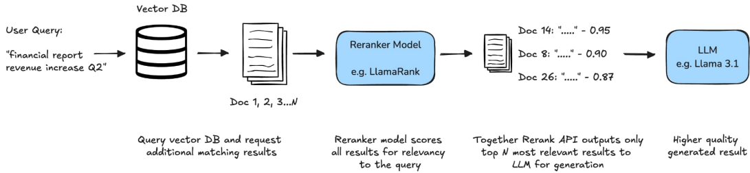
Figure 4.8: Reranker [138].
