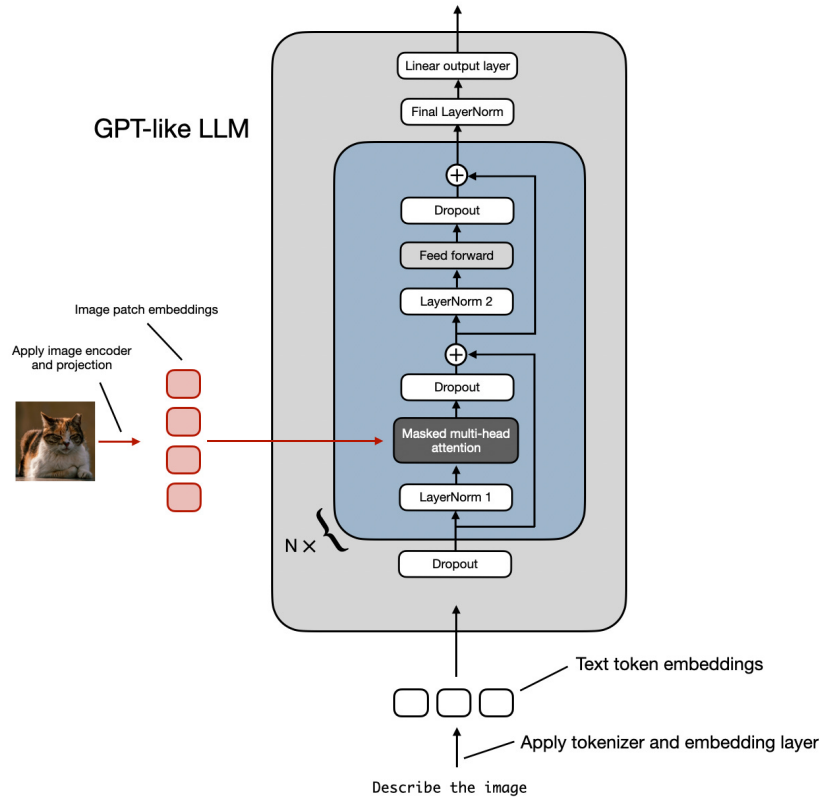
Figure 4.4: Cross-attention [42].
