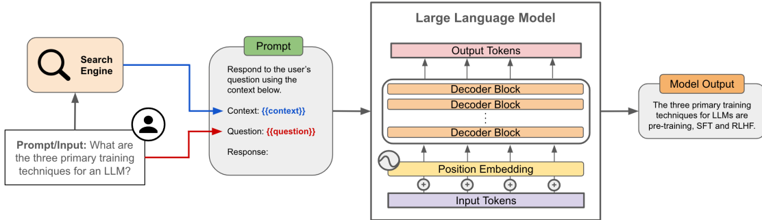
Figure 4.10: Generator [147]
