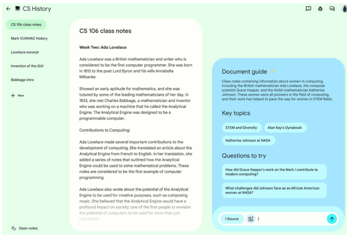
Figure 5.1: NotebookLM [173].
