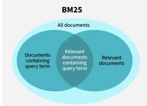
Figure 4.7: BM25 [130].
