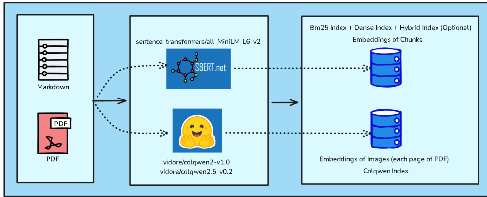
Figure 6.5: Dual-Stream Indexing Layer.
