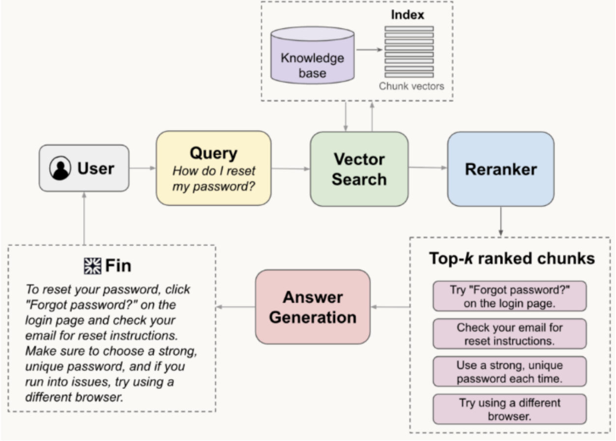
Figure 2.8: Reranker [together2024_rerank_llamarank].
