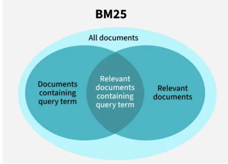
Figure 2.7: BM25 [geeksforgeeks_bm25].
