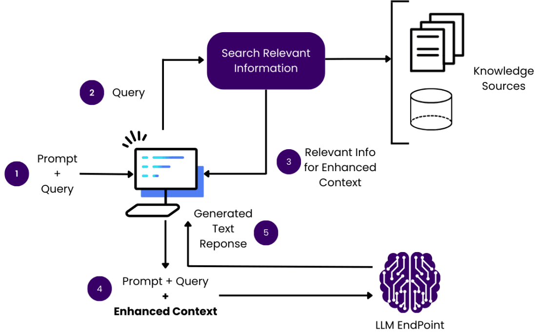
Figure 2.9: Augmentation [obot_rag_guide]
