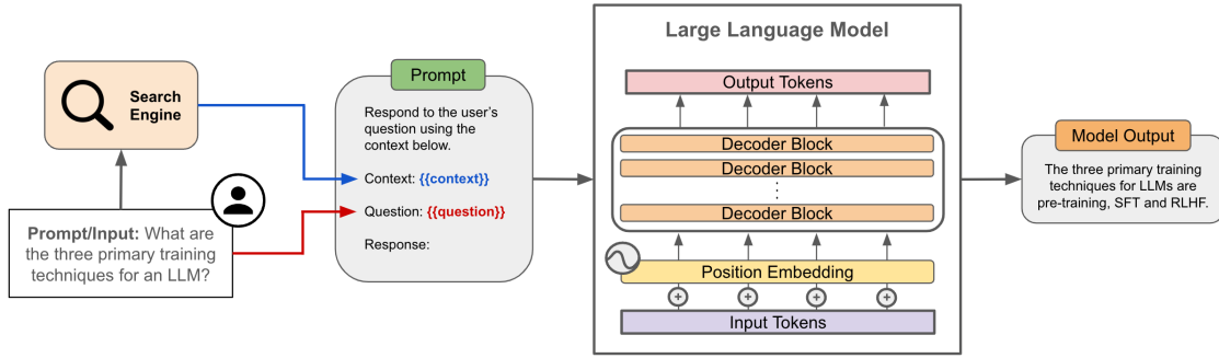
Figure 2.10: Generation [wolfe2024_rag_guide]
