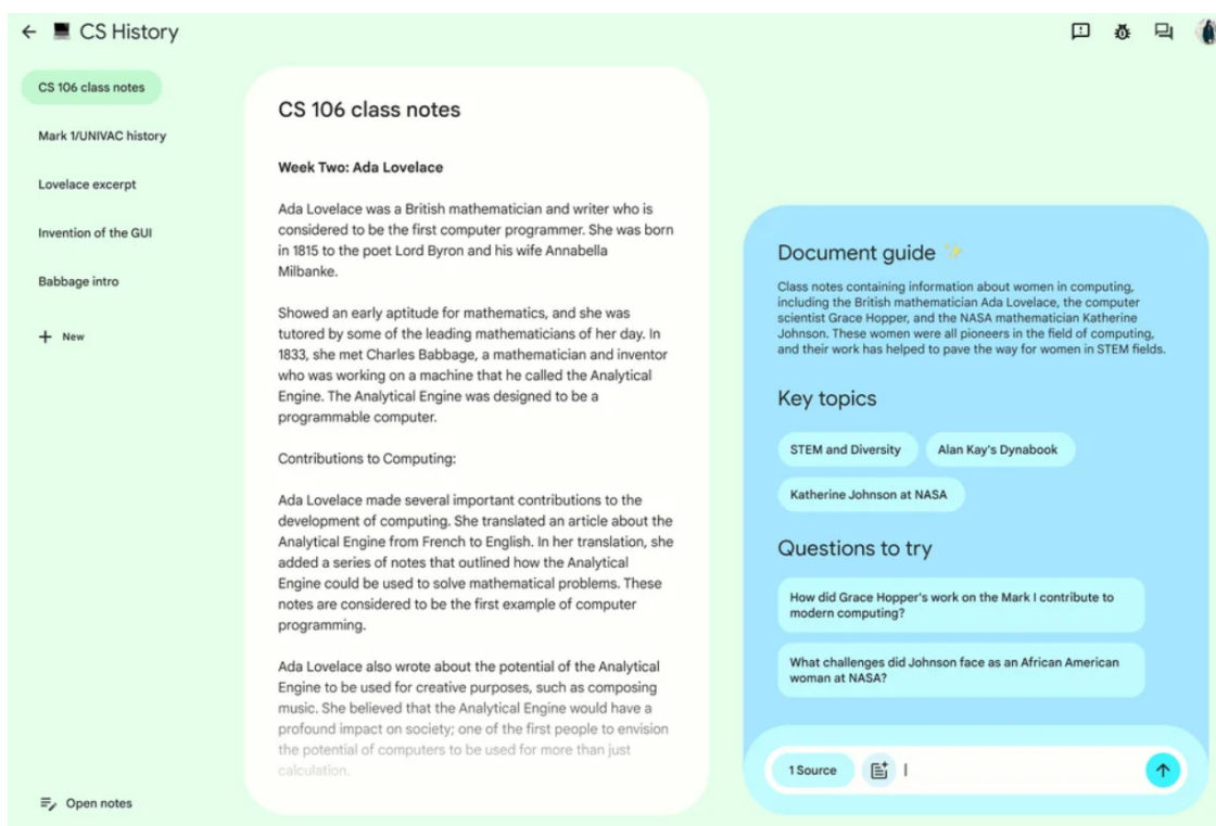
Figure 3.1: NotebookLM [notebooklm-google-ai].
