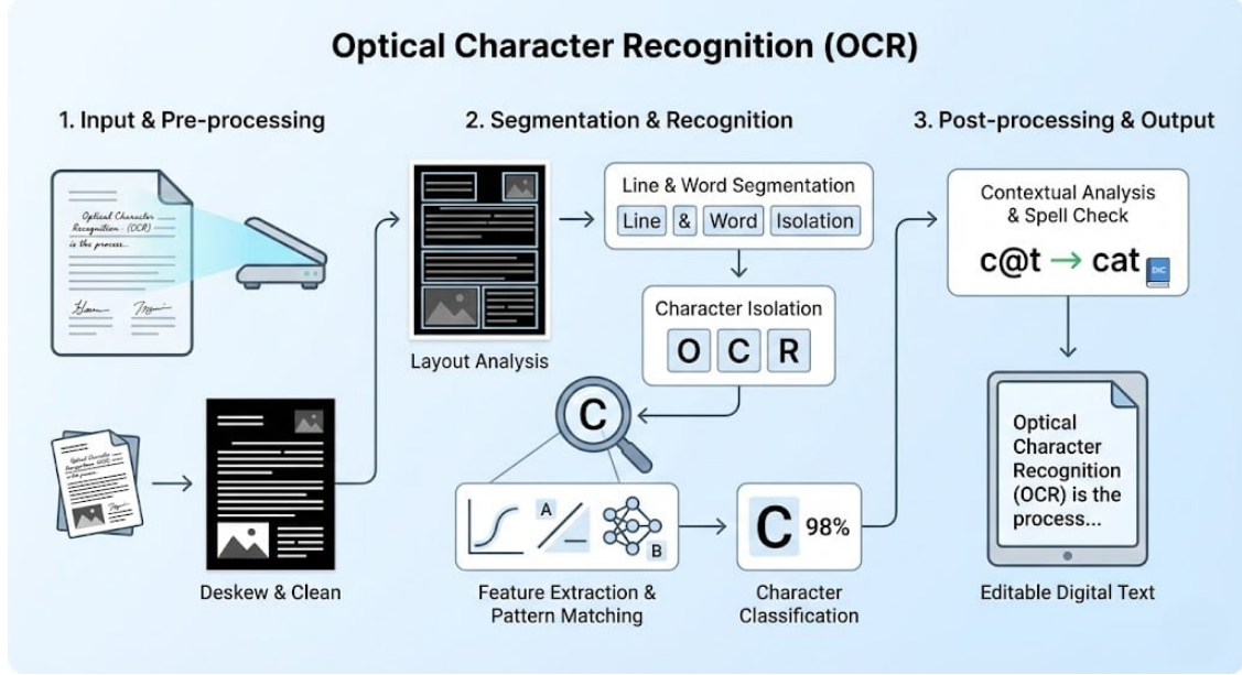
Figure 2.2: OCR pipeline.
