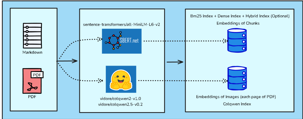
Figure 4.2: Dual-Pathway Embedding and Indexing Architecture.
