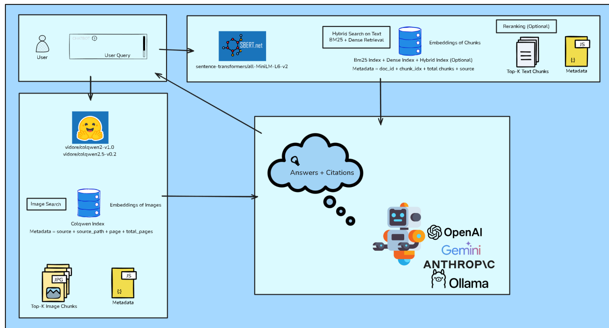
Figure 4.8: Overall System Architecture.
