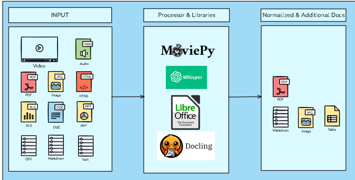
Figure 4.1: Data Processing Pipeline Normalization Stage.
