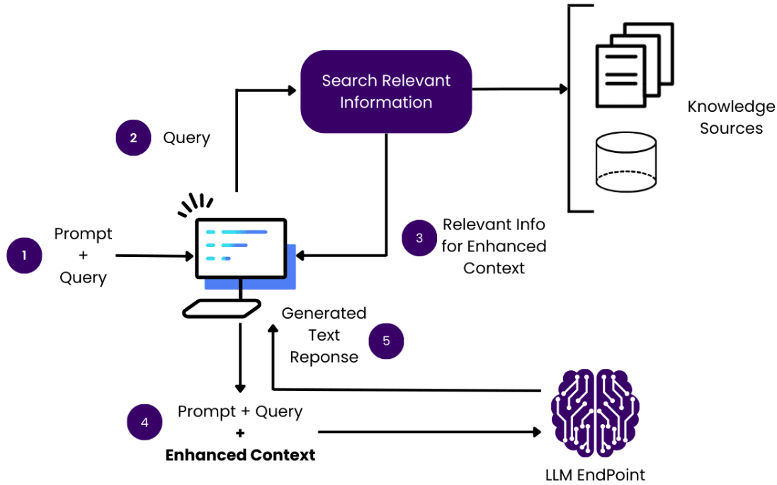
Figure 2.9: Augmentation
