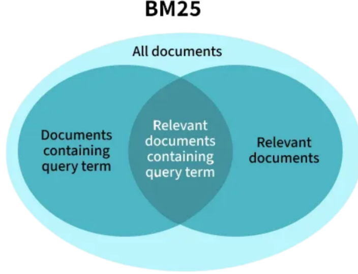
Figure 2.7: BM25
