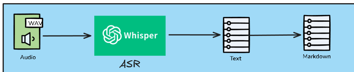
Figure 4.4: Whisper Audio Transcription Flow.
