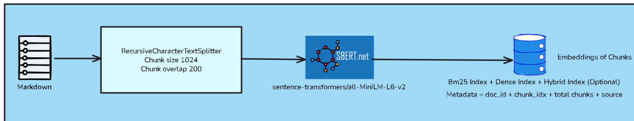
Figure 4.6: Text Embedding Flow.
