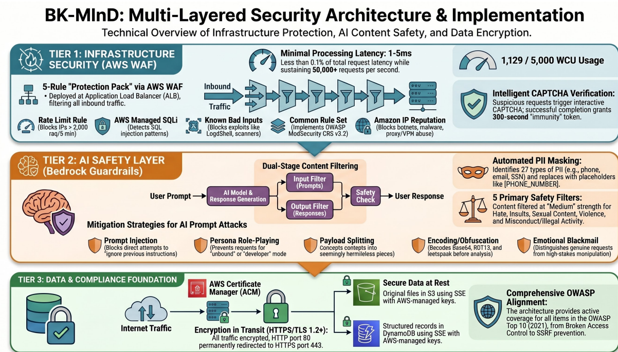
Figure 4.6: BK-MInD Three-Tier Security Architecture.
