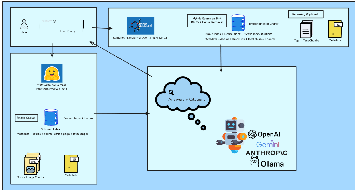
Figure 4.5: Overall MRAG System Architecture: Retrieval and Generation Flow.
