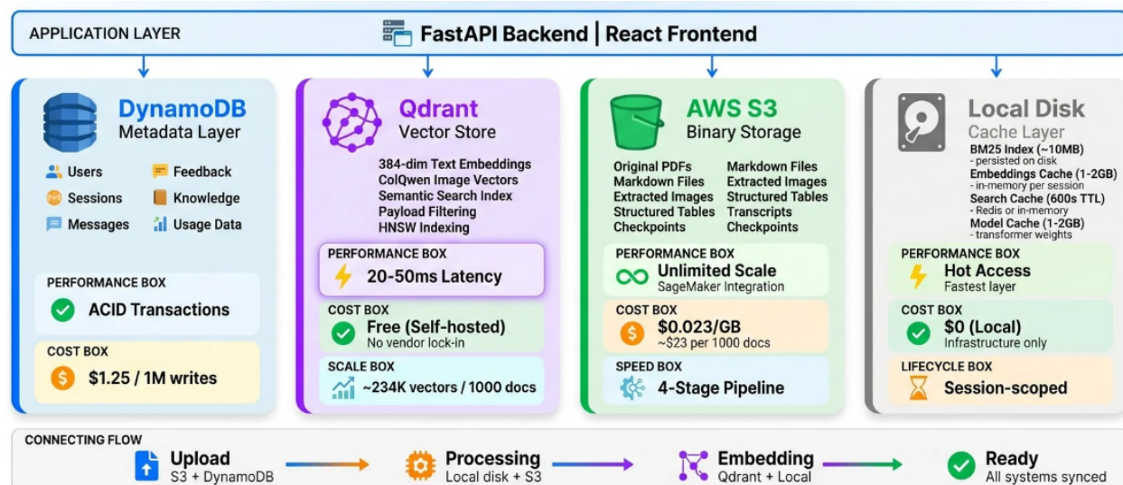
Figure C.15: 4-layer storage system: specialized databases for each data type.
