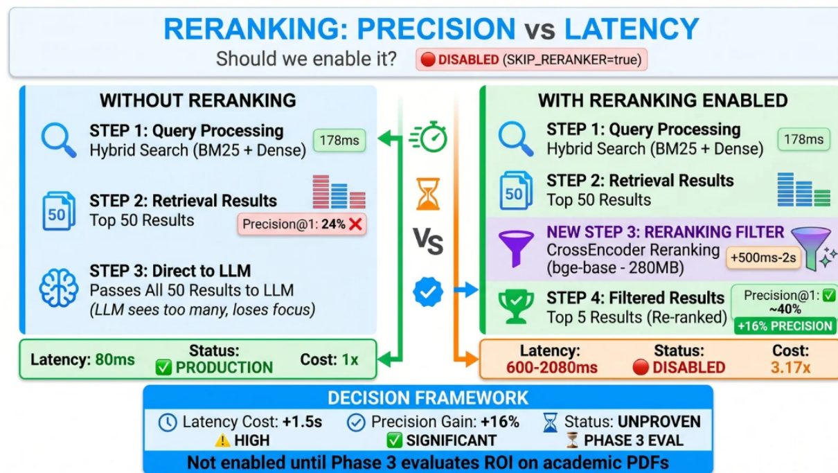
Figure C.14: Reranking trade-off: precision vs. latency comparison.
