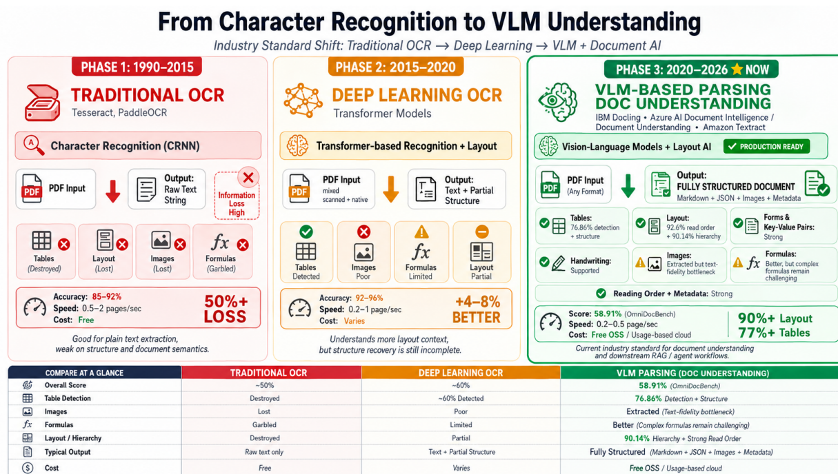
Figure C.16: Three generations of document parsing: OCR evolution.
