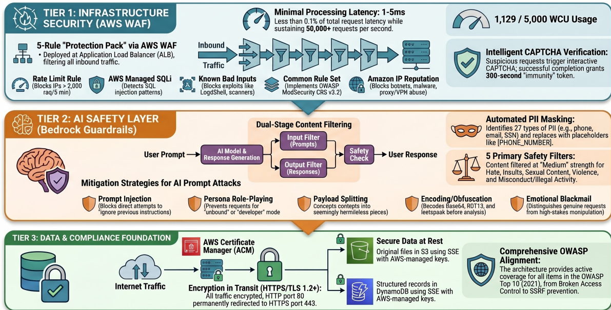
Figure 5.18: Multi-layered security architecture combining WAF, Bedrock Guardrails, and data encryption.
