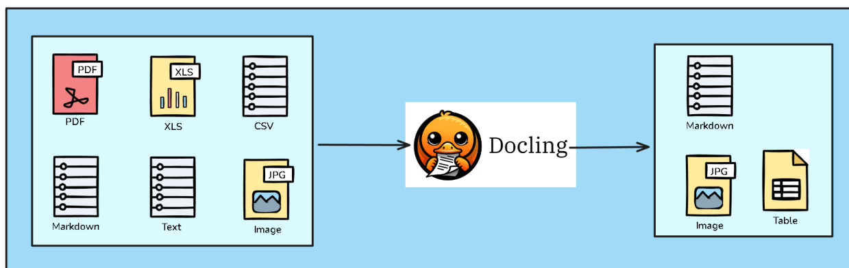
Figure 7.4: Docling Document Parsing Process.
