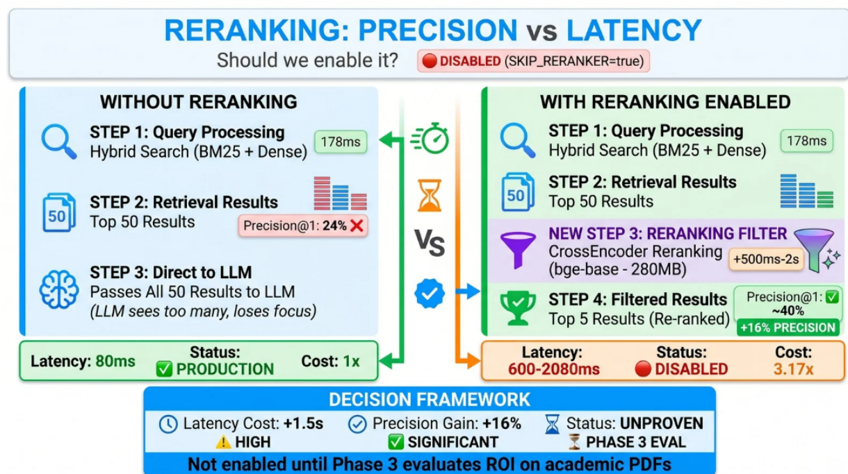
Figure C.1: Reranking trade-off: precision vs. latency comparison.
