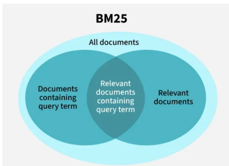
Figure 2.7: BM25 [geeksforgeeks_bm25].
