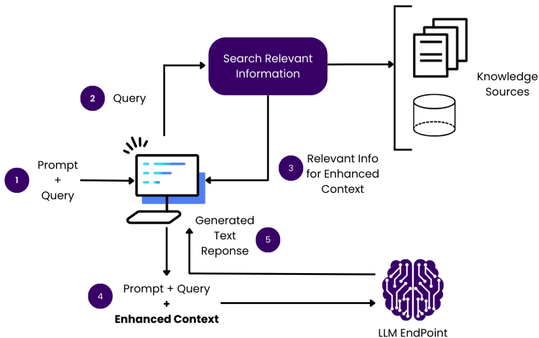
Figure 2.9: Augmentation [obot_rag_guide]
