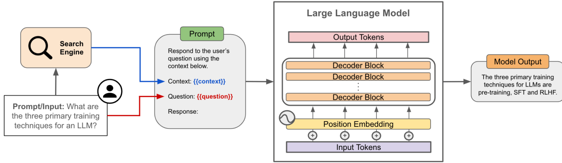
Figure 2.10: Generation [wolfe2024_rag_guide]
