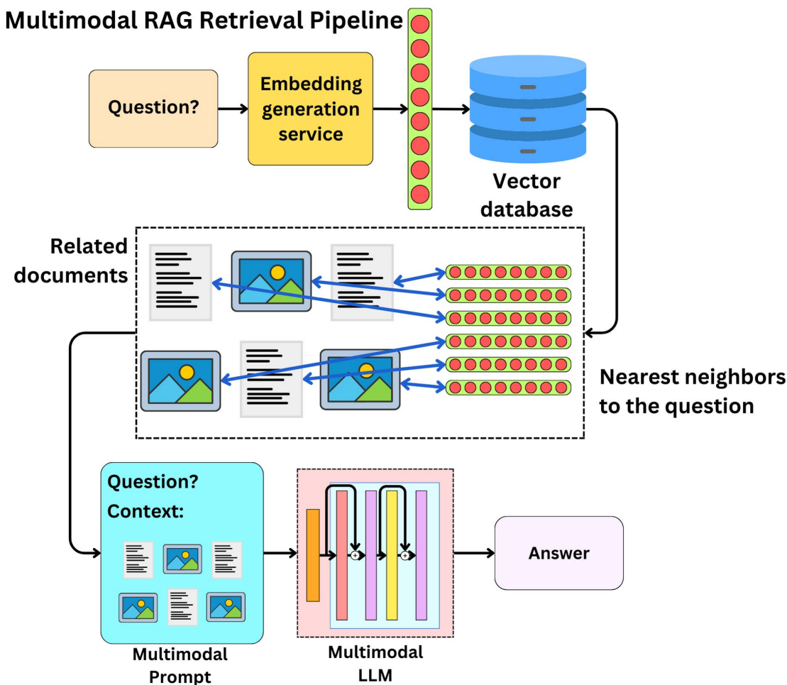
Figure 2.6: MRAG pipeline.
