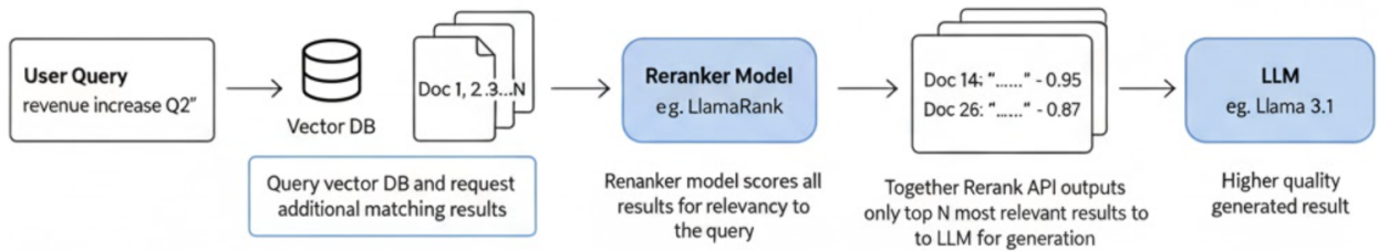
Figure 2.7: Reranker.
