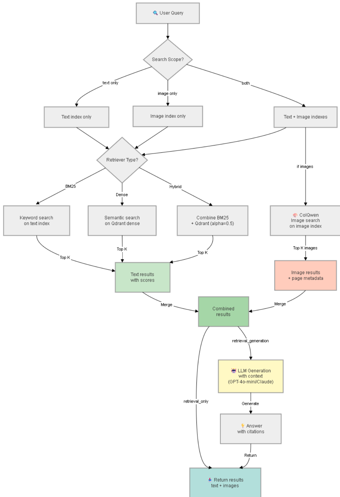
Figure 5.11: Search and Retrieval Pipeline Flow.
