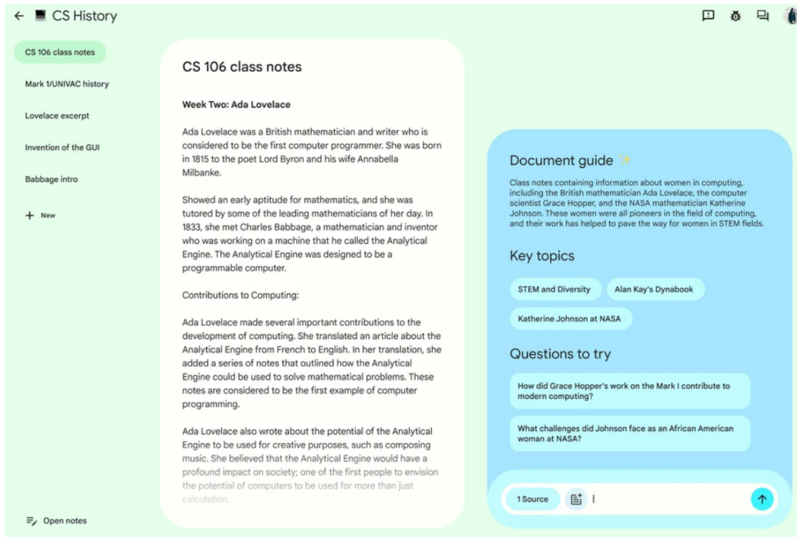
Figure 3.1: NotebookLM.
