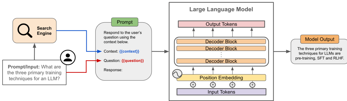
Figure 2.9: Generation.
