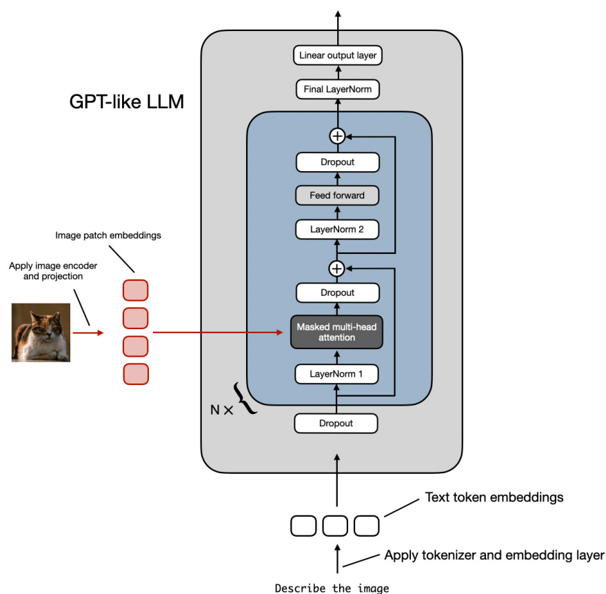
Figure 2.4: Cross-attention.
