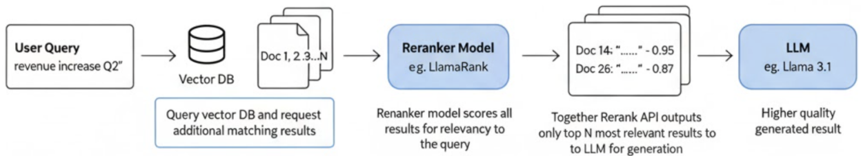
Figure 2.7: Reranker.
