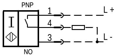
3RG4023-3AB00-PF / 3RG4023-2AB00-PF:
