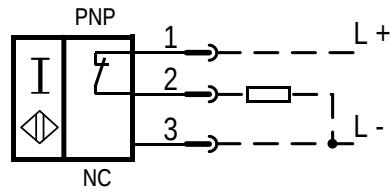
3RG4023-3AA00-PF / 3RG4023-2AA00-PF:
