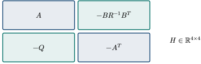
Figure 4: The block layout of Equation 16 for the running example, each block labeled by the problem data it carries. The diagonal blocks A and -A^T mirror each other; the off-diagonal blocks -G and -Q are symmetric – this is the matrix-level image of “antisymmetric times symmetric.”
