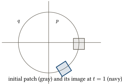
Figure 2: One small square patch of the phase plane at t = 0 (gray, near q = 1.1, p = -0.05 ) and its image under the flow at t = 1 (navy). The patch rides a rotation by one radian around the energy circle (light gray) and lands as a rotated square of the same area – which Equation 6 guarantees, since a rotation preserves every area.
