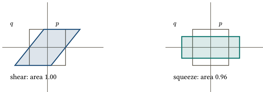
Figure 1: The unit square (gray) sent through two area-preserving-looking maps. The shear (navy) is symplectic: every parallelogram area, including the square's, survives. The squeeze (teal) multiplies all areas by 0.96, and its form defect \|M^T J M - J\| = 0.04 detects exactly that.
