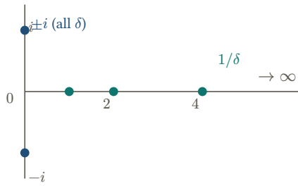
Figure 1: The spectrum of the example as \delta falls. The complex pair stays at \pm i ; the third eigenvalue is 1/\delta , moving right and reaching infinity at \delta = 0 . Inspect that only the third eigenvalue moves: tuning \delta changes the conditioning of B , not the oscillator.
