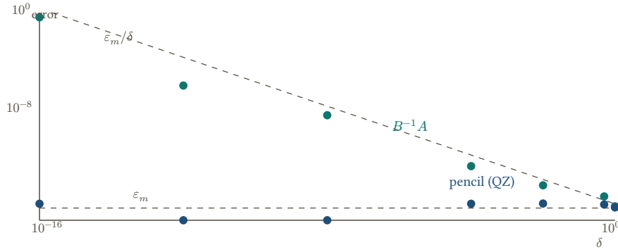
Figure 2: The same table as a picture, on logarithmic axes. The teal series (the ratio route B^{-1}A ) rises along the steep dashed guide \varepsilon_m/\delta as \delta falls: the digits lost are roughly the digits of 1/\delta . The navy series (the pencil route) lies on the machine-precision floor, the horizontal dashed line at \varepsilon_m . Numbers from scripts/verify_qz.m .
