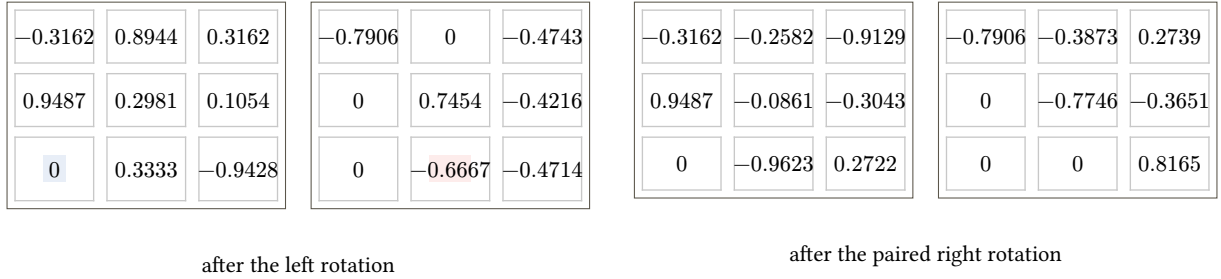
Figure 4: The paired rotations of phase two, on the running example from scripts/qz_sweeps.m . Panel 1: after the left rotation, A 's entry (3, 1) is gone (navy) and B has gained the single entry (3, 2) (rose). Panel 2: the right rotation clears B(3, 2) and leaves A 's zero alone, because it operates on columns 2 and 3 while the zero is in column 1. The result is Hessenberg over triangular.
