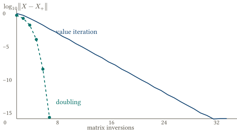
Figure 3: Error against the work, on Equation 3. The horizontal axis counts matrix inversions – one per value-iteration step, one per squaring. The navy curve is the value iteration; the teal markers are the doubling iterates, which are the same errors reached at work k instead of 2^k . The value iteration is a straight line of slope \log_{10} 0.531 ; the doubling curve steepens because each step squares the previous error. On this problem the value iteration needs 27 inversions to reach X_+ and doubling needs six.
