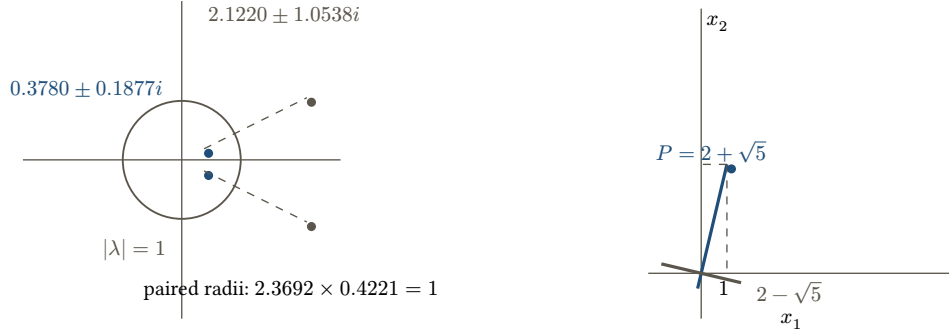
Figure 7: Why the discrete criterion is the unit circle, and what is read off. Left: the eigenvalues of the deflated pencil for the double integrator below, drawn by scripts/dare_sweeps.m ; they come in reciprocal pairs about the unit circle, so selecting the ones inside it is a complete rule, and each selected eigenvalue is exactly a closed-loop pole. Right: the two eigenvector directions of the scalar pencil in the state plane. The stable direction is the graph of P : its slope is the answer, and the dashed guides read that slope off as P = 2 + \sqrt{5} . The other direction is the unstable eigenvector, whose slope is the other root's value 2 - \sqrt{5} .
