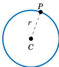
(a) Circle: center C , radius r = \text{constant}
