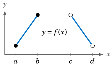
Figure 3.3.3 Extreme Value Theorem
