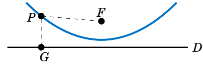
Figure 7.3.3 Hyperbola: \frac{PF}{PG} = e > 1
