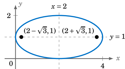
Figure 7.4.2 Ellipse \frac{(x-2)^2}{4} + (y-1)^2 = 1
