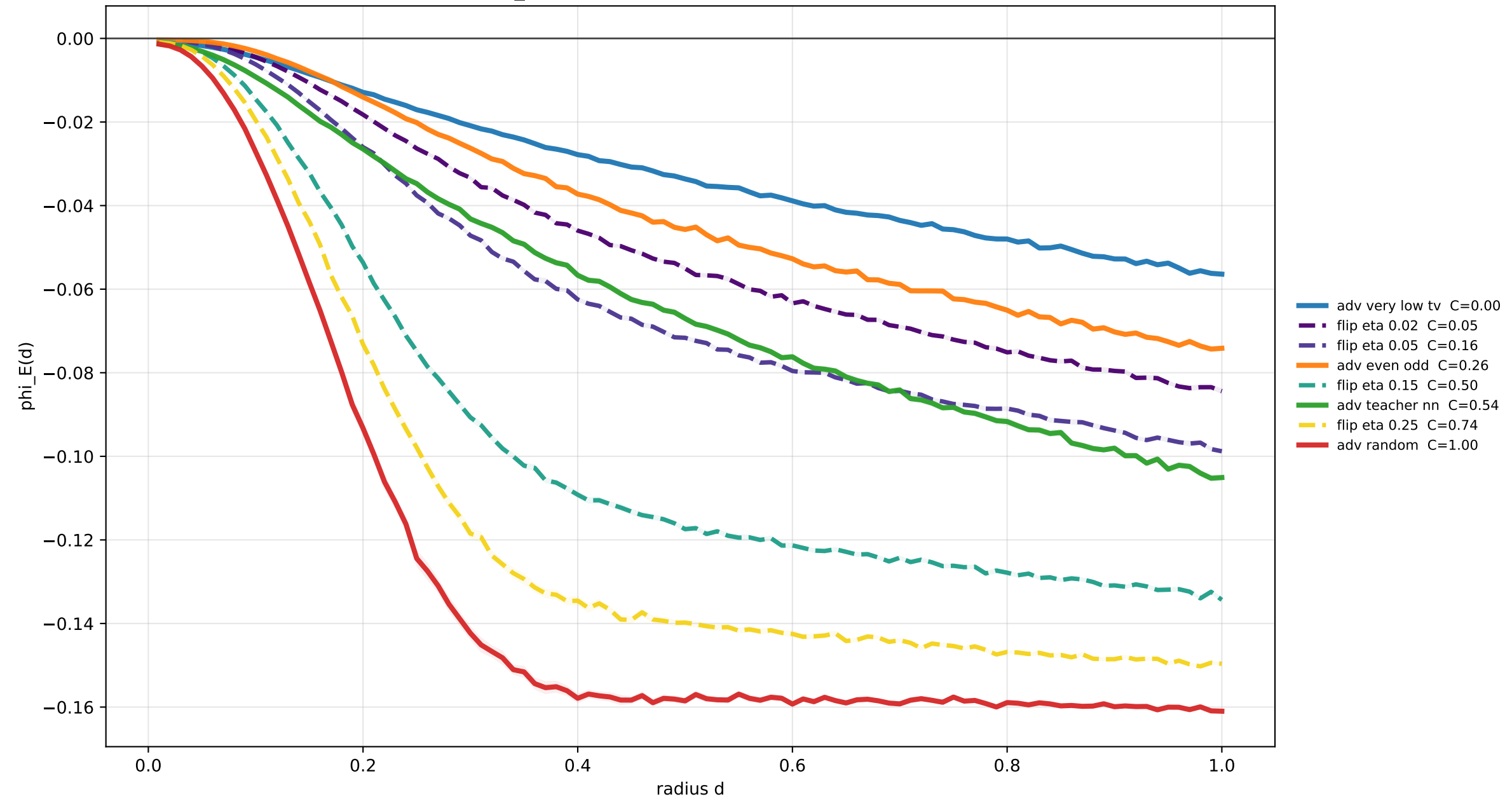
MNIST \phi_E curves ordered by empirical complexity C
