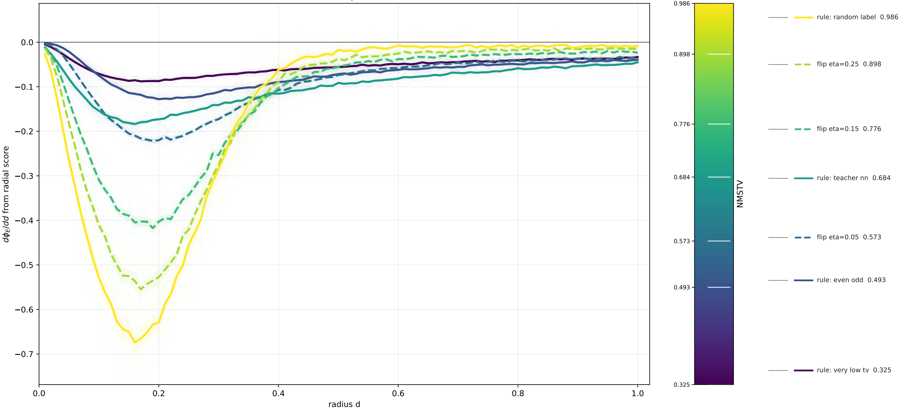
MNIST active rules + eta flips: direct first derivative
