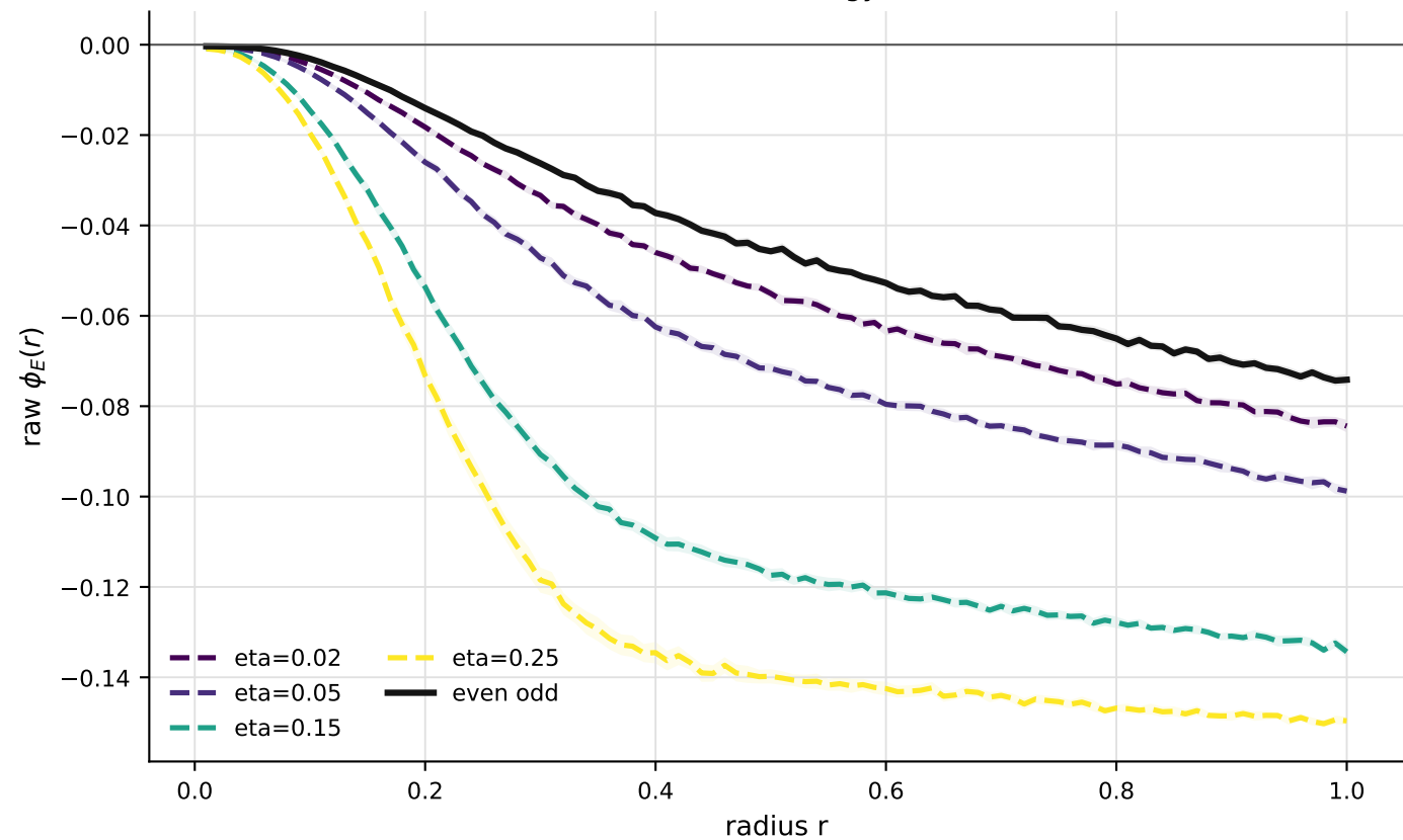
Raw local free-energy curves
