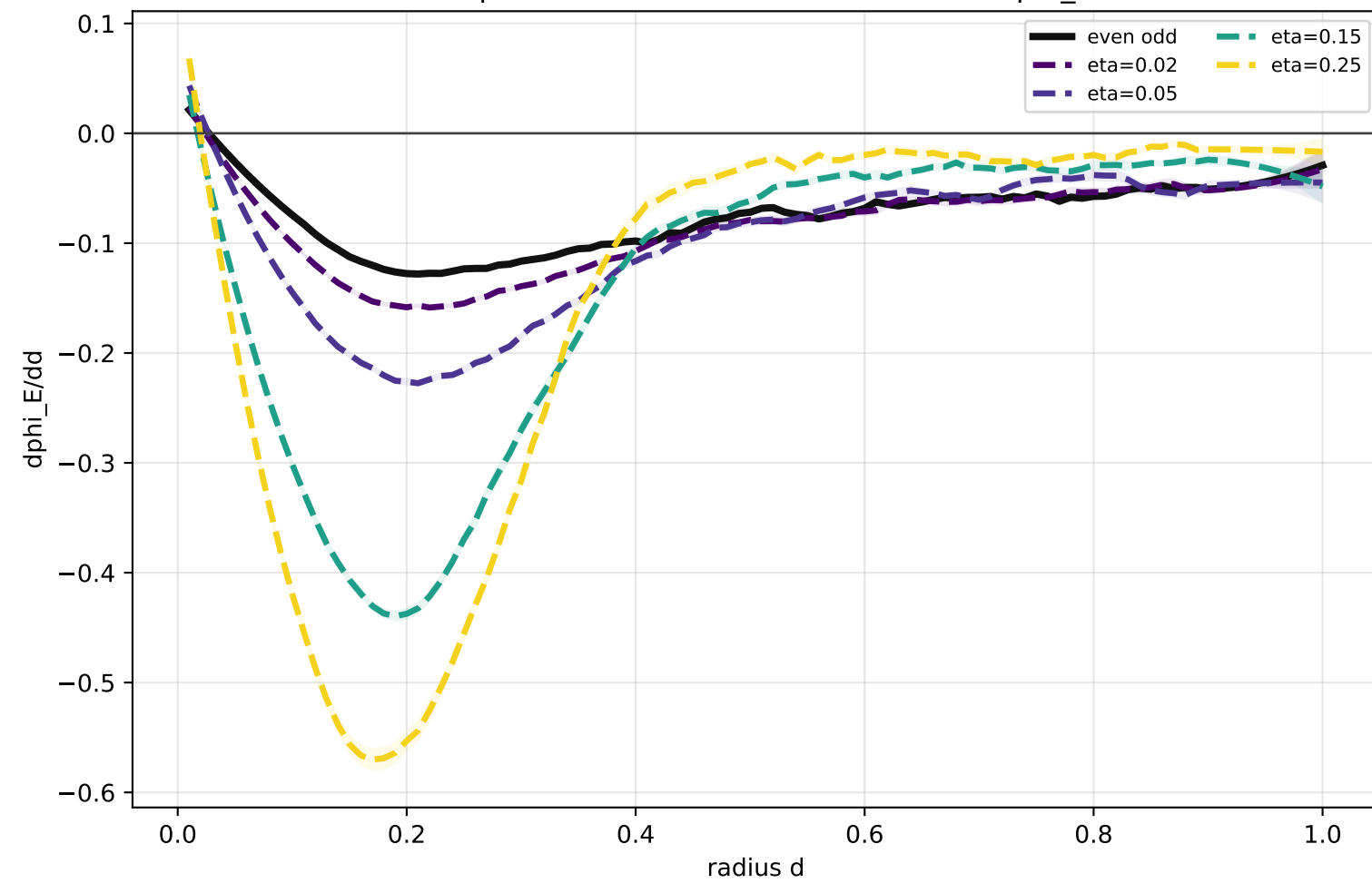
MNIST A_\kappa : smooth crossover, not collapse
