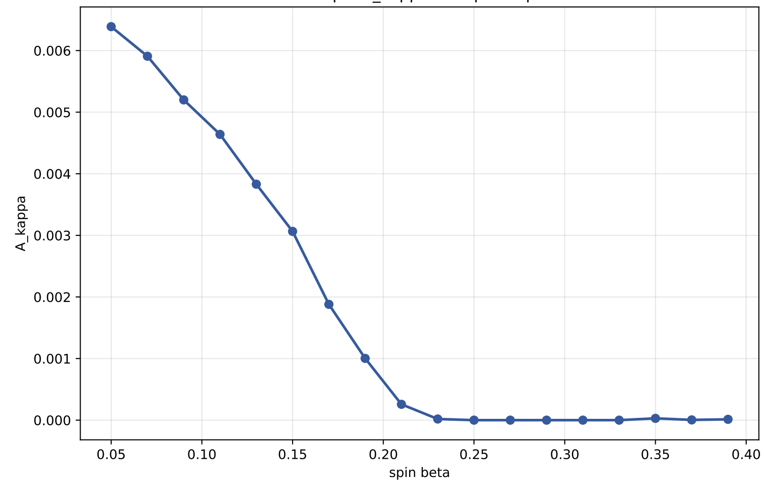
3NN spin A_\kappa : sharp collapse
