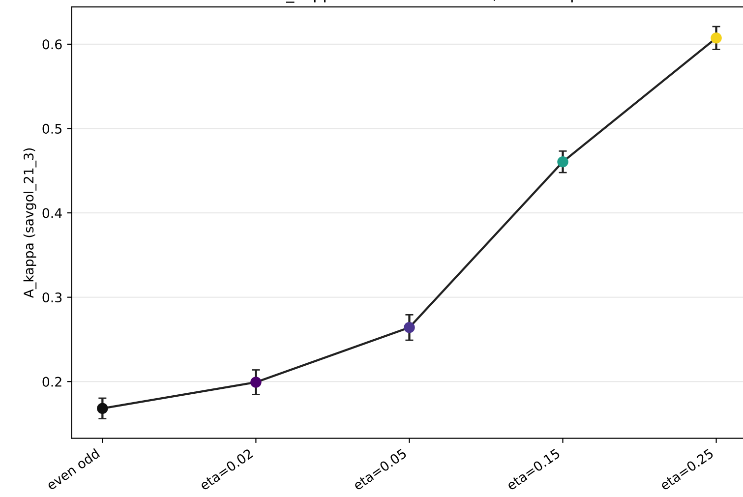
MNIST A_\kappa : smooth crossover, not collapse
