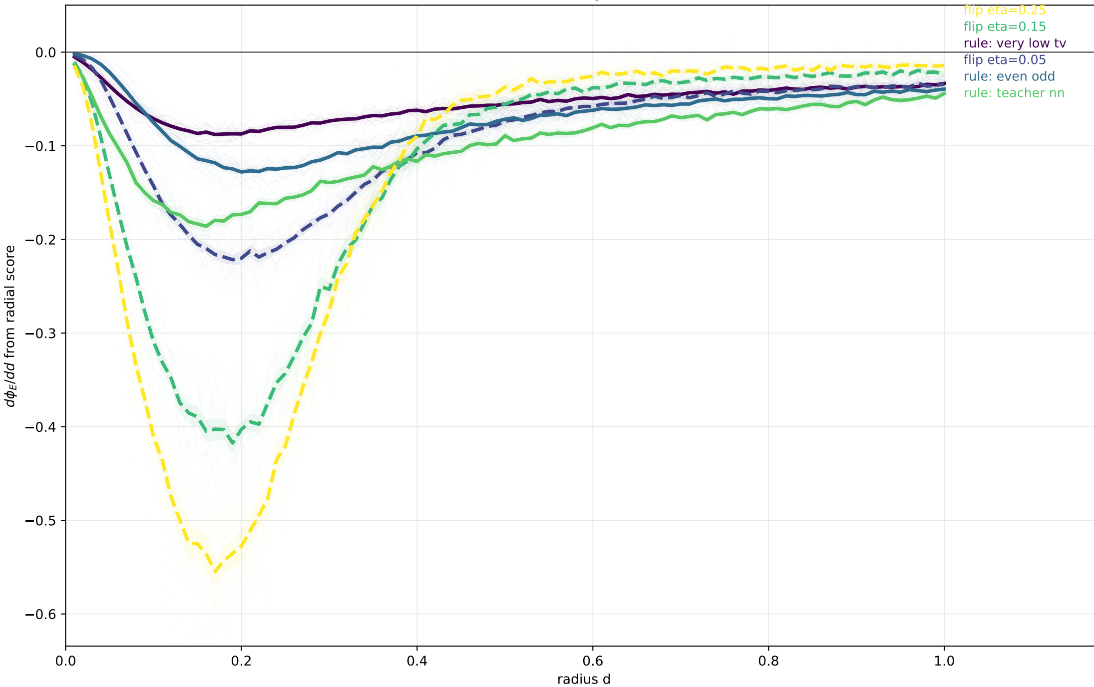
MNIST active rules + eta flips: direct first derivative
