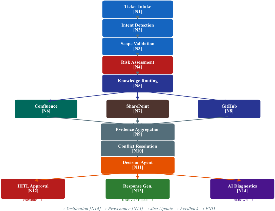
Fig. 7.7 — ORION-AI LangGraph 15-Node Multi-Agent Pipeline (ticket_intake → intent_detection → ... → feedback [END])
