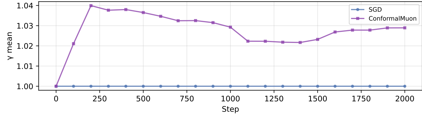
blocks.1.ln1 — \gamma trajectory
