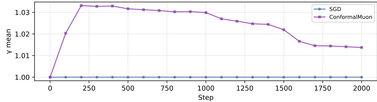
blocks.2.ln1 — \gamma trajectory
