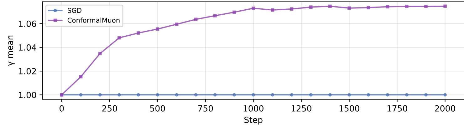
blocks.2.ln2 — \gamma trajectory
