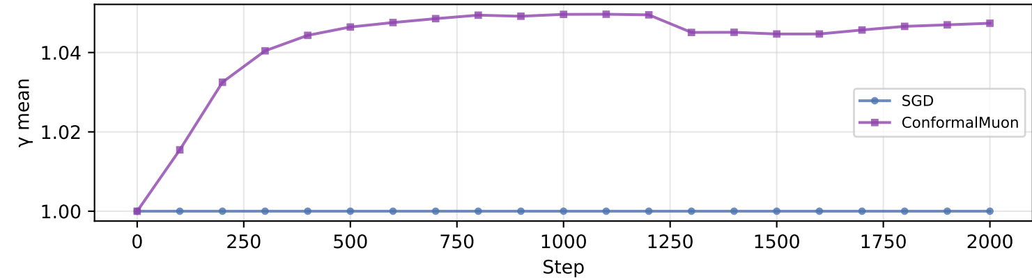
blocks.1.ln2 — \gamma trajectory
