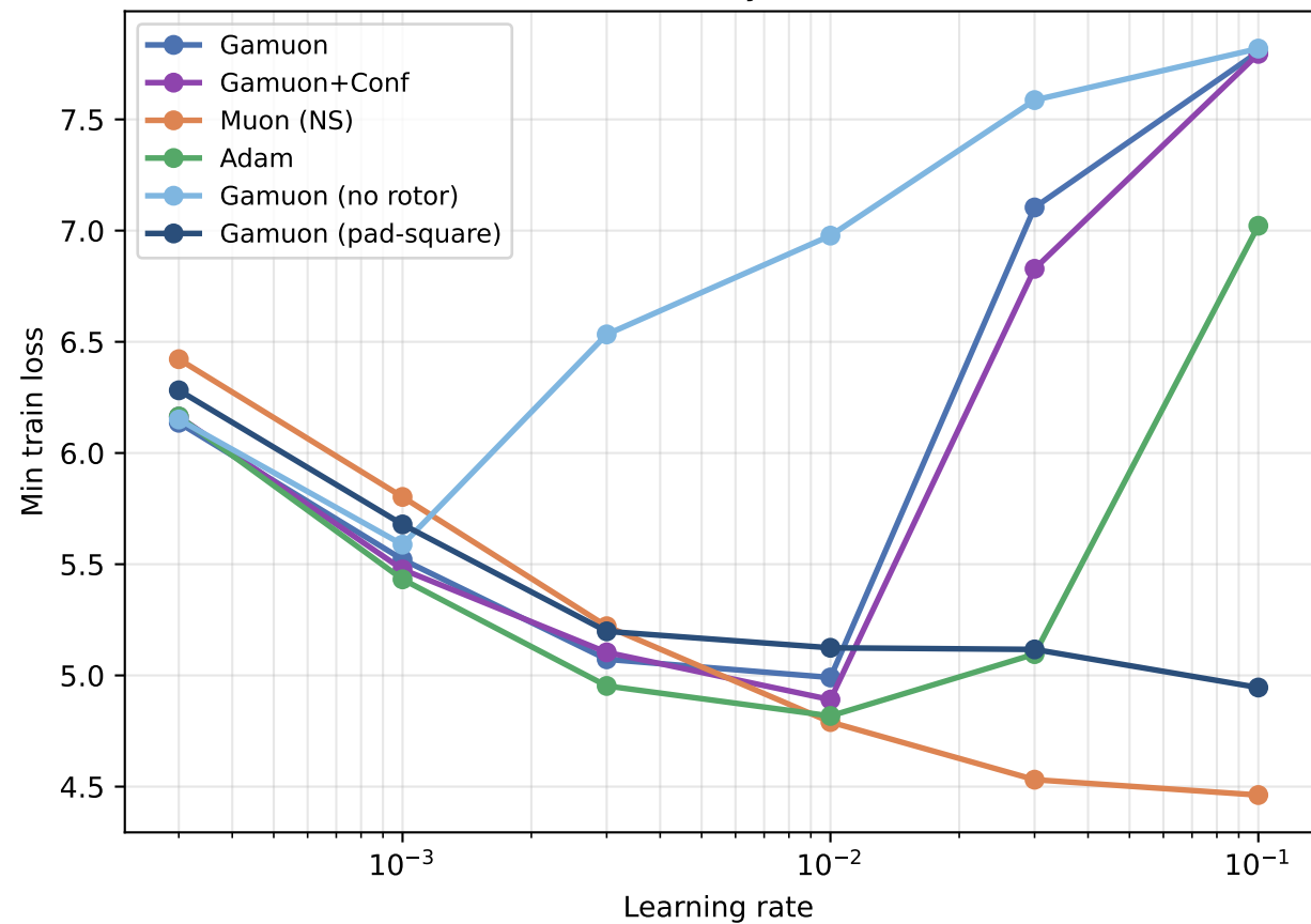
LR sensitivity — train
