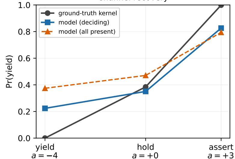
Channel recovery
