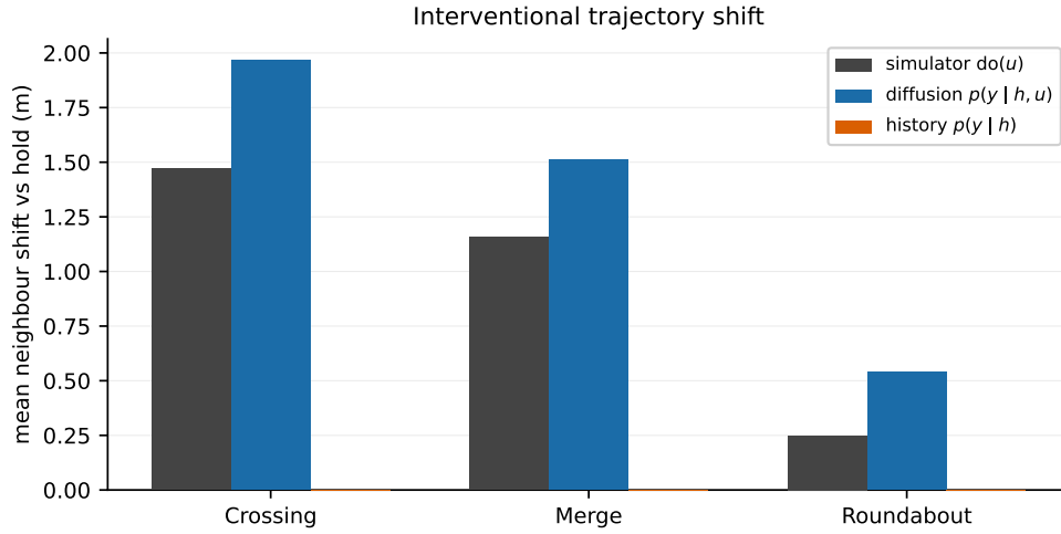
Fig. 13. Interventional neighbour shift versus the hold plan. History cannot move with u (shift identically zero). Diffusion overshoots the simulator slightly but has the correct sign on every map.
