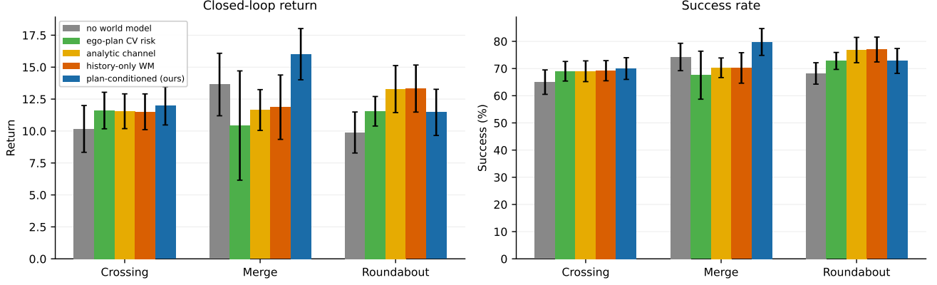
Fig. 6. Closed-loop return and success on all three maps (mean \pm s.d. over seeds). Geometry captures most of the lift on the crossing; plan-conditioned diffusion is the outlier on the merge; kernel and history lead on the roundabout.
