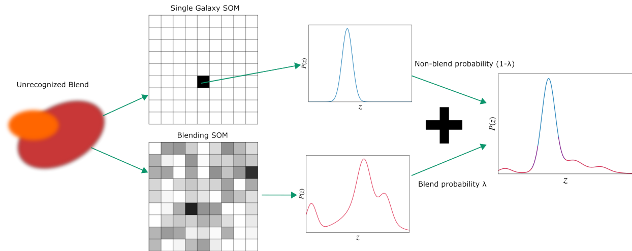
Figure 3: Example of modeling blends when producing redshift estimates via a SOM. Instead of only using the cell of the best fit, a weighted SOM can be made from synthetic blends that can be used to produce a more accurate PDF (color-coded to highlight contribution from individual terms).
