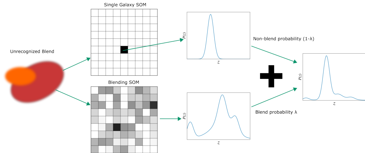
Figure 3: Example of modeling blends when producing redshift estimates.
