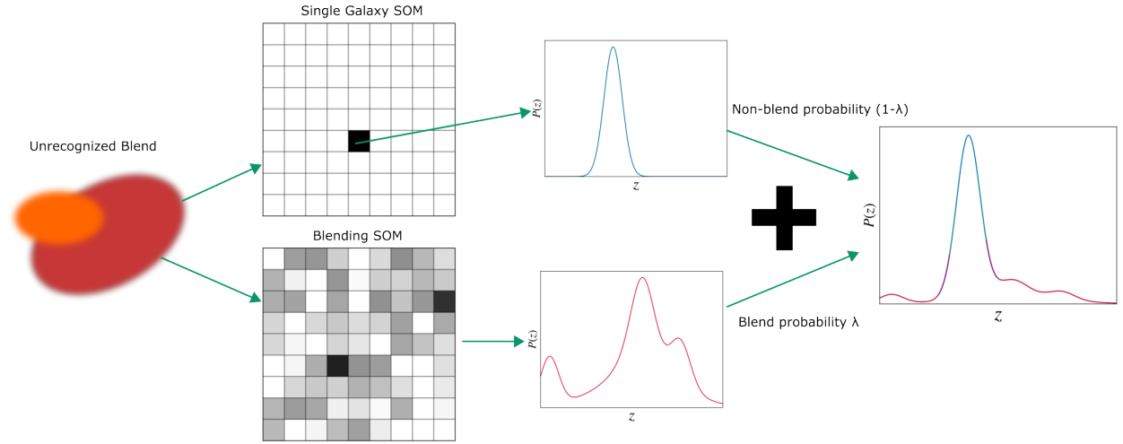
Figure 3: Example of modeling blends when producing redshift estimates via a SOM. Instead of only using the cell of the best fit, a weighted SOM can be made from synthetic blends that can be used to produce a more accurate PDF (color-coded to highlight contribution from individual terms).
