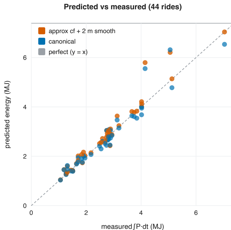
Figure 2. Predicted vs measured ride energy for the two best models, one point per ride. Both hug the identity line (dashed); the shared over-prediction on the two highest-energy rides is
