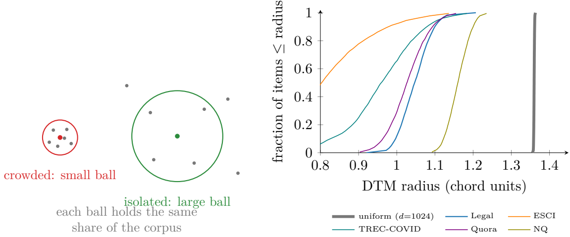
Figure 7: The distance-to-measure field. Left : the intuition schematic — each item is scored by the radius of the ball it needs to gather a fixed share ( m = 2\% ) of the corpus. Right : the field’s exact CDF on the real corpus (measured): the entire field sits left of the uniform needle at 1.36, and the finding is the low tail against the corpus’s own bulk (1st percentile 0.966 against median 1.047), whose members the instrument names by id (Figure 8); the text explains why the uniform band reads on the cone rather than on pockets. The four grid corpora under the same encoder overlay their CDFs: each has its own bulk position and low-tail mass — per-item crowding profiles differ far more across corpora than any global statistic suggests.
