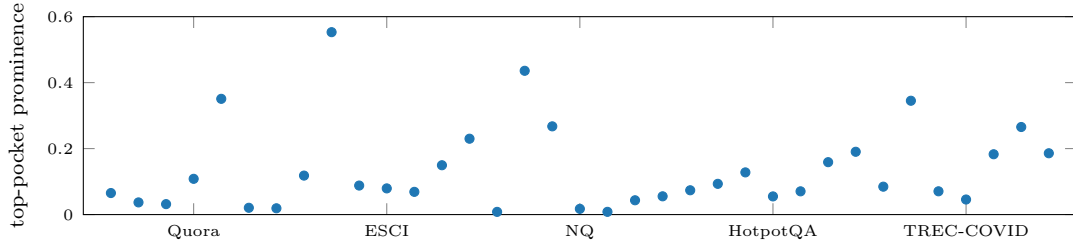
Figure 17: Structure across the grid: the most prominent pocket’s merge-tree prominence for every corpus–encoder cell (all 35 exceed the null-calibrated floor). The spread within each corpus is as large as the spread across corpora: encoders disagree about which corpora form tight substructure. The text draws the consequence.
