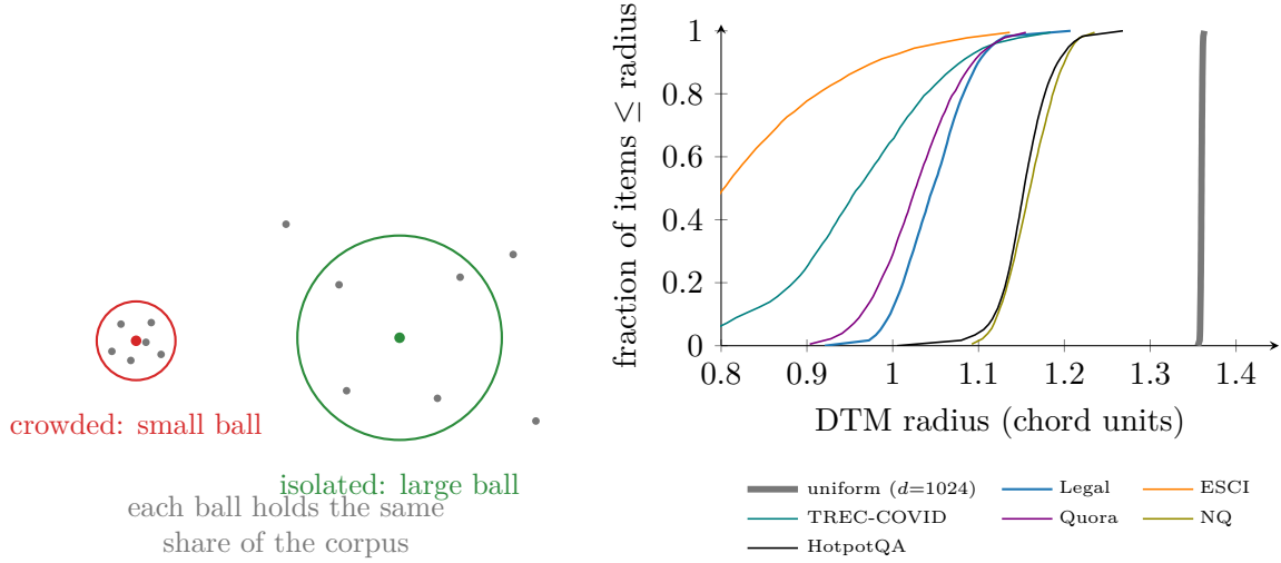
Figure 7: The distance-to-measure field. Left : the intuition schematic — each item is scored by the radius of the ball it needs to gather a fixed share ( m = 2\% ) of the corpus. Right : the field’s exact CDF on the real corpus (measured): the entire field sits left of the uniform spike at 1.36, and the finding is the low tail against the corpus’s own bulk (1st percentile 0.966 against median 1.047), whose members the instrument names by id (Figure 8); the text explains why the uniform band reads on the cone rather than on pockets. The five grid corpora under the same encoder overlay their CDFs: each has its own bulk position and low-tail mass — per-item crowding profiles differ far more across corpora than any global statistic suggests.
