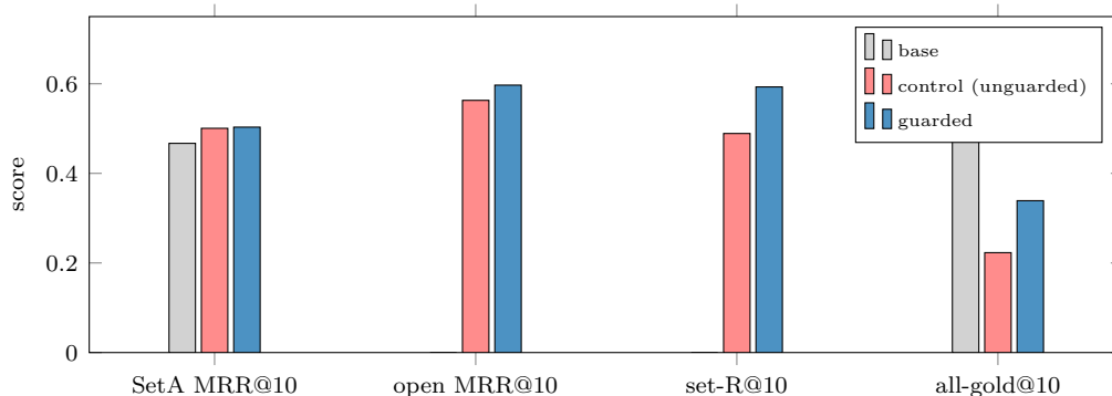
Figure 14: The guardrail experiment on the frozen evaluations. On the target task (Set A MRR@10) the guarded arm matches the control — the guardrails are free. On the untar- geted open evaluation the guarded arm wins every metric, most sharply on the multi-hop all-gold@10 where the control reproduces the historical regression (base \approx 0.48 , historical baseline; base bars for the open single/set metrics were not measured under this harness and are omitted).
