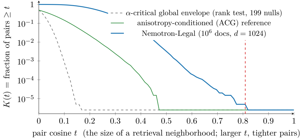
Figure 5: The crowding curve on the real corpus (Nemotron-Legal [58], computed from the report’s own 2 \times 10^5 -pair sample). Through mid-similarities the data track the anisotropy-matched reference — that excess over uniformity is the cone, benign — but above \cos \approx 0.8 the curve rises above both references: genuine tight-pair structure, globally significant at the minimum attainable p = 1/200 . No bin width or lattice placement exists anywhere in the figure, and the liftoff claim is family-wise valid across all scales.
