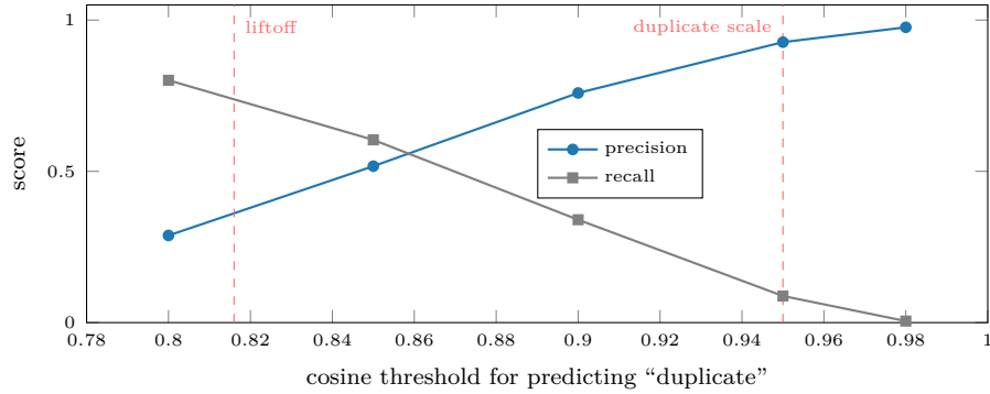
Figure 16: Duplicate prediction from pair cosine alone on Quora’s annotated duplicate pairs (case-study encoder; 15,675 gold pairs). Precision rises monotonically toward the duplicate scale — the ground-truth reading of “the closer to one, the more surely duplicate” — while recall falls, because annotated duplicates are mostly paraphrases living between the liftoff and duplicate scales: the confusable window.
