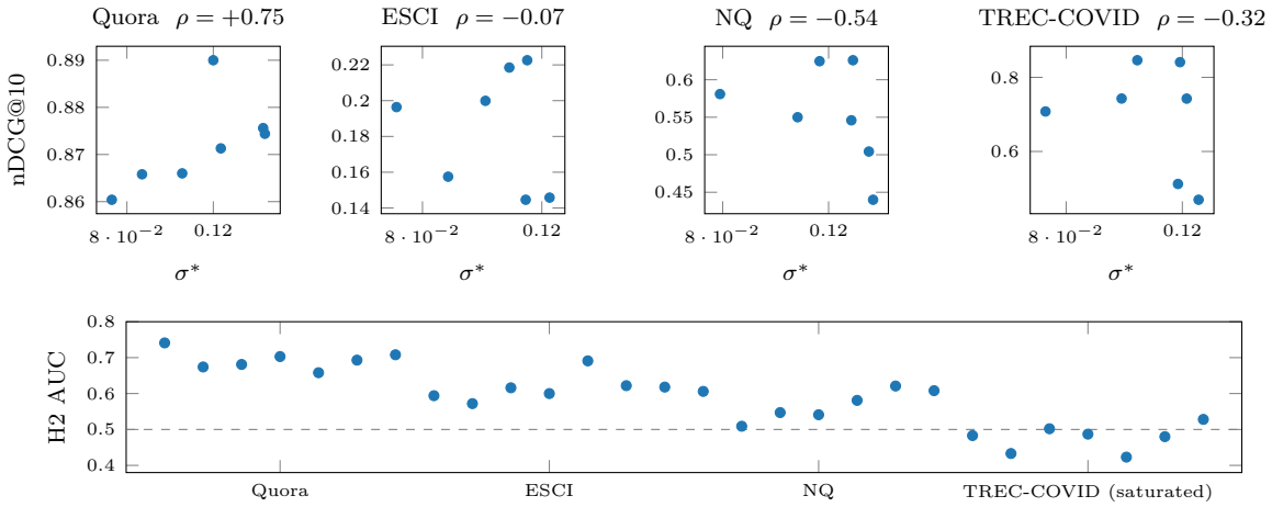
Figure 15: Every grid cell, plotted. Top: within each corpus, the seven encoders’ \sigma^* against their nDCG@10 — rank correlation is strongly positive only where relevance is geometric matching (Quora), null on product search, and negative where semantic competence gaps dominate. Bottom: the per-document collision field’s failure-prediction AUC for all 28 cells, grouped by corpus, against the chance line — above 0.5 in every informative cell; the TREC-COVID group is uninformative because its outcome label saturates (98% of judged documents past rank 10).
