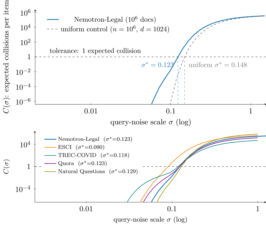
Figure 11: Expected collisions vs. query noise on the real corpus (measured; Nemotron-Legal). The curves separate exactly in the decision region — the corpus’s cone and tight pairs dominate C(\sigma) at the noise scales where retrieval operates, pulling the tolerance crossing from \sigma^* = 0.148 to 0.123: the corpus retains 83% of a well-spread corpus’s noise budget. At large \sigma the curves converge (every pair confuses) and at tiny \sigma both vanish; the tolerance crossing is determined where they differ. The lower panel overlays the five corpora under the same encoder: the ordering and spacing of their \sigma^* values (0.090 to 0.129) is the corpus-side noise-budget comparison the instrument is designed to support. On the traced benchmark the same construction attributes a cost of 26% of the budget to the planted 5% pocket ( \sigma^*: 0.203 \rightarrow 0.150 ).
