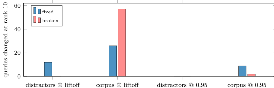
Figure 14: The routing dissociation as counts (values from Table 12). At the liftoff scale, removing foreign confusable material only fixes; merging within the formulaic corpus at that same scale mostly breaks. At the true-duplicate scale the pattern reverses in both sites. Each repair is licensed at exactly one scale and one site — the mapping the instrument’s readouts prescribe.
