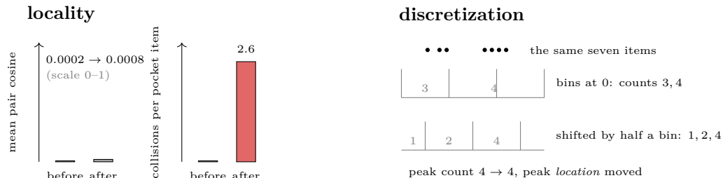
Figure 1: The two measurement difficulties, previewed (schematic; the left panel’s numbers are the traced benchmark’s, §4). Left: planting 200 near-duplicates in 4,000 items moves the corpus-wide average by 0.0006 on a scale of 1, while each planted item’s expected retrieval collisions rise from \approx 0 to 2.6 — the pathology is severe and local, so per-item readouts see what averages cannot. Right: binning the same seven items with the same bin width but a half-bin origin shift changes the counts and relocates the peak — the discretization, not the data, chose the answer. §5 quantifies this on the tool’s own displays.
