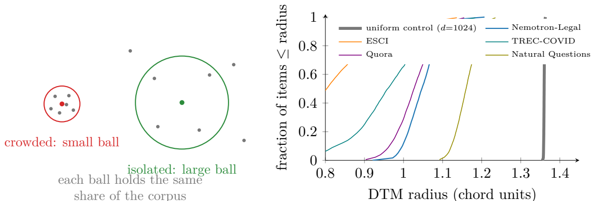
Figure 6: The distance-to-measure field. Left : the intuition schematic — each item is scored by the radius of the ball it needs to gather a fixed share ( m = 2\% ) of the corpus. Right : the field’s exact CDF on the real corpus (measured): the entire field sits left of the uniform needle at 1.36 — the anisotropy cone shortens every radius, so the uniform band is diagnostic of the cone, not of pockets — and the finding is the low tail against the corpus’s own bulk (1st percentile 0.966 against median 1.047), whose members the instrument names by id (Figure 7). The four grid corpora under the same encoder overlay their CDFs: each has its own bulk position and low-tail mass — per-item crowding profiles differ far more across corpora than any global statistic suggests.
