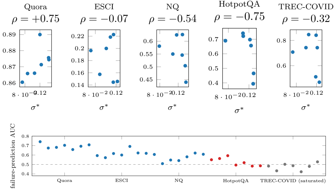
Figure 16: Every grid cell, plotted. Top: within each corpus, the seven encoders’ \sigma^* (horizontal) against their nDCG@10 (vertical) — rank correlation is strongly positive only where relevance is geometric matching (Quora), null on product search, and negative where semantic competence gaps dominate. Bottom: the per-document collision field’s failure-prediction AUC for all 35 cells, grouped by corpus, against the chance line. It sits above 0.5 in every informative cell outside the multi-hop group (red), where three of seven encoders fall to chance; the TREC-COVID group (gray) is uninformative because its outcome label saturates (98% of judged documents past rank 10).
