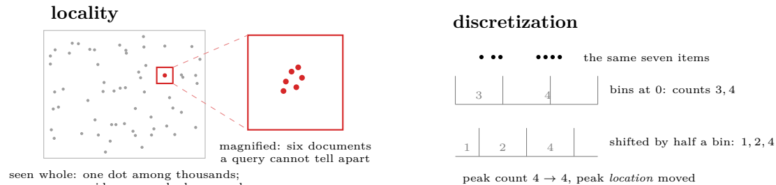
Figure 1: The two measurement difficulties, previewed (schematic). Left: viewed whole, the corpus shows nothing unusual — the defect is one dot among thousands, and on the benchmark of §4, inserting 200 near-duplicates into 4,000 items moves mean pairwise similarity by only \approx 0.002 on a scale of 1 (§2.3). Magnified, that dot is six documents a query cannot tell apart, each expecting 2.6 retrieval collisions against zero for a well-spread corpus. The pathology is severe, local, and invisible to any average. Right: binning the same seven items with the same bin width but a half-bin origin shift changes the counts and relocates the peak — the discretization, not the data, chose the answer. §5 quantifies this on the tool’s own displays.
