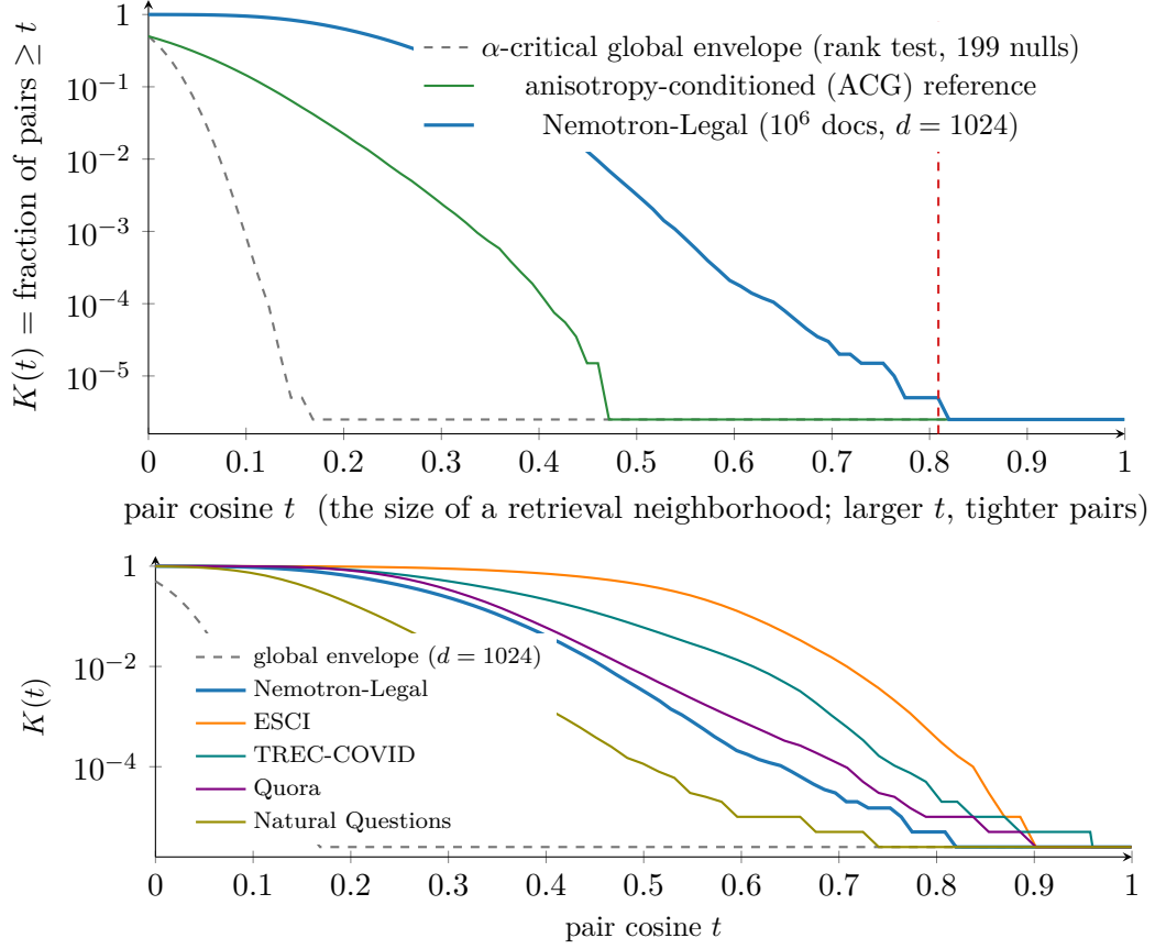
Figure 5: The crowding curve on the real corpus (Nemotron-Legal [58], computed from the report’s own 2 \times 10^5 -pair sample). Through mid-similarities the data track the anisotropy-matched reference — that excess over uniformity is the cone, benign — but above \cos \approx 0.8 the curve rises above both references: genuine tight-pair structure, globally significant at the minimum attainable p = 1/200 . No bin width or lattice placement exists anywhere in the figure, and the liftoff claim is family-wise valid across all scales. Bottom: the same curve for five corpora under the same encoder ( d = 1024 , shared envelope) — every corpus carries tight-pair mass far above the null, with distinct anatomies: ESCI and TREC-COVID hold the most near-duplicate mass, Quora the least beyond its paraphrase band.
