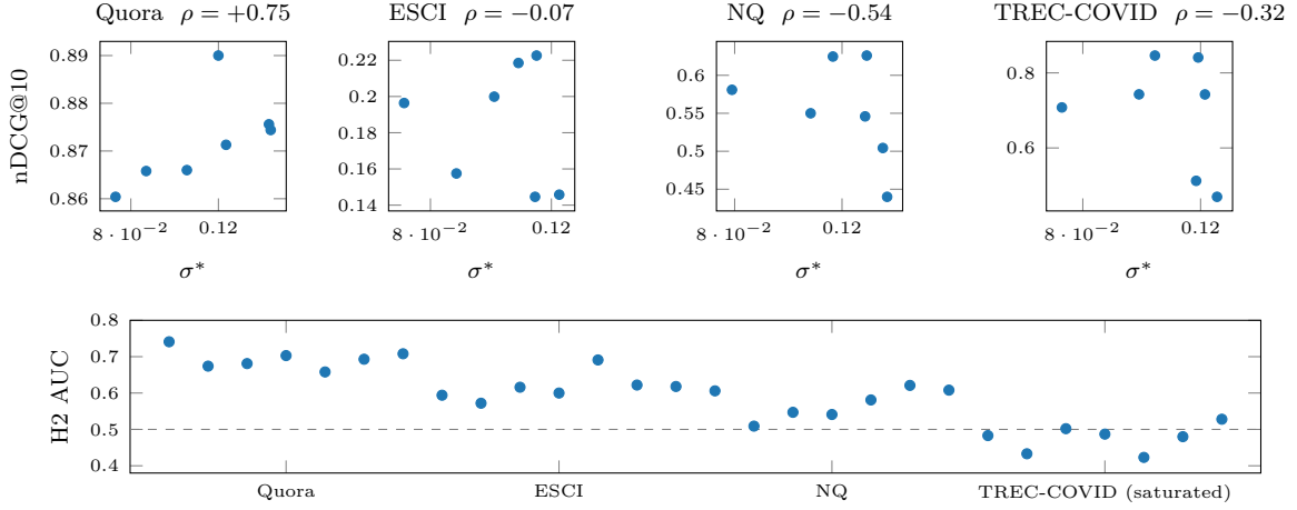
Figure 15: Every grid cell, plotted. Top: within each corpus, the seven encoders’ \sigma^* against their nDCG@10 — rank correlation is strongly positive only where relevance is geometric matching (Quora), null on product search, and negative where semantic competence gaps dominate. Bottom: the per-document collision field’s failure-prediction AUC for all 28 cells, grouped by corpus, against the chance line — above 0.5 in every informative cell; the TREC-COVID group is uninformative because its outcome label saturates (98% of judged documents past rank 10).
