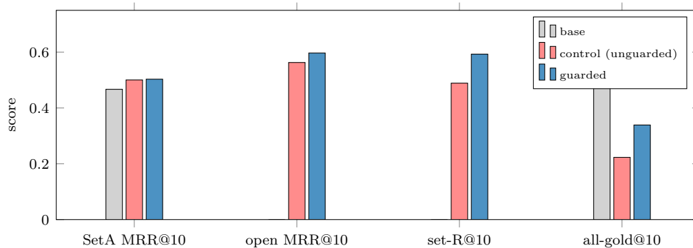
Figure 14: The guardrail experiment on the frozen evaluations. On the target task (Set A MRR@10) the guarded arm matches the control — the guardrails are free. On the untar-geted open evaluation the guarded arm wins every metric, most sharply on the multi-hop all-gold@10 where the control reproduces the historical regression (base \approx 0.48 , historical baseline; base bars for the open single/set metrics were not measured under this harness and are omitted).
