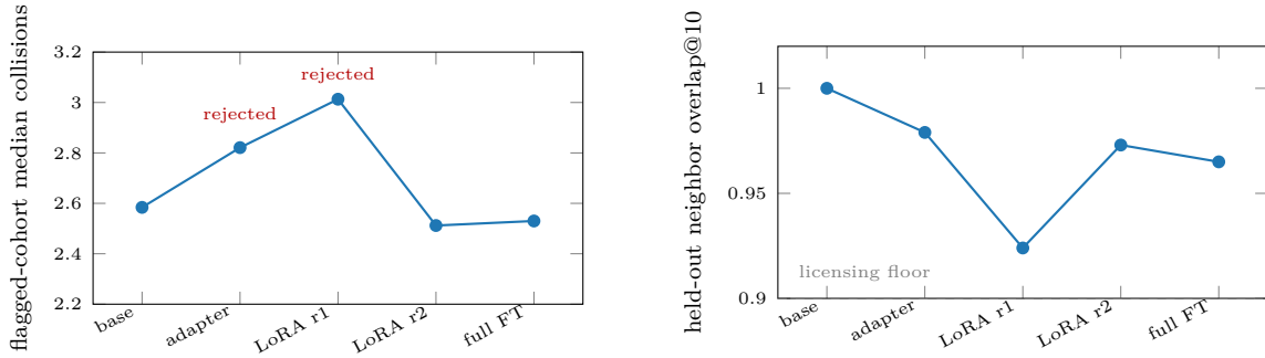
Figure 12: The encoder loop’s held-out verdicts by round (values from Table 11). Left: median expected collisions of the flagged cohort, tracked at fixed \sigma — the two rejected rounds worsen the cohort while their training losses decreased; the corrected rounds improve it. Right: neighbor overlap against the base model, with the pre-registered licensing floor; every accepted round stays above it.
