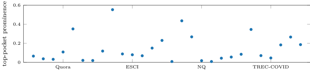
Figure 16: Structure across the grid: the most prominent pocket’s merge-tree prominence for every corpus-encoder cell (all 28 exceed the null-calibrated floor). The spread within each corpus is as large as the spread across corpora — encoders disagree strongly about which corpora form tight substructure, which is precisely why pocket findings must be read per corpus-encoder pair rather than as corpus properties.
