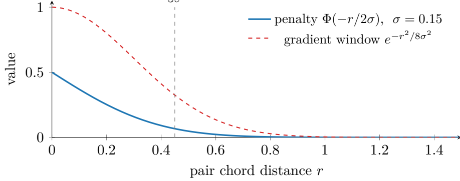
Figure 11: The confusion loss’s gradient locality at a measured \sigma = 0.15 (the benchmark’s \sigma^* ): all gradient lives inside the confusable window; pairs beyond \approx 3\sigma are exponentially untouched. “Improve resolution without disturbing dissimilarity” is a property of the kernel, not a hope.
