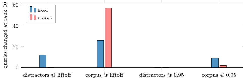
Figure 13: The routing dissociation as counts (values from Table 12). At the liftoff scale, removing foreign confusable material only fixes; merging within the formulaic corpus at that same scale mostly breaks. At the true-duplicate scale the pattern reverses in both sites. Each repair is licensed at exactly one scale and one site — the mapping the instrument’s readouts prescribe.
